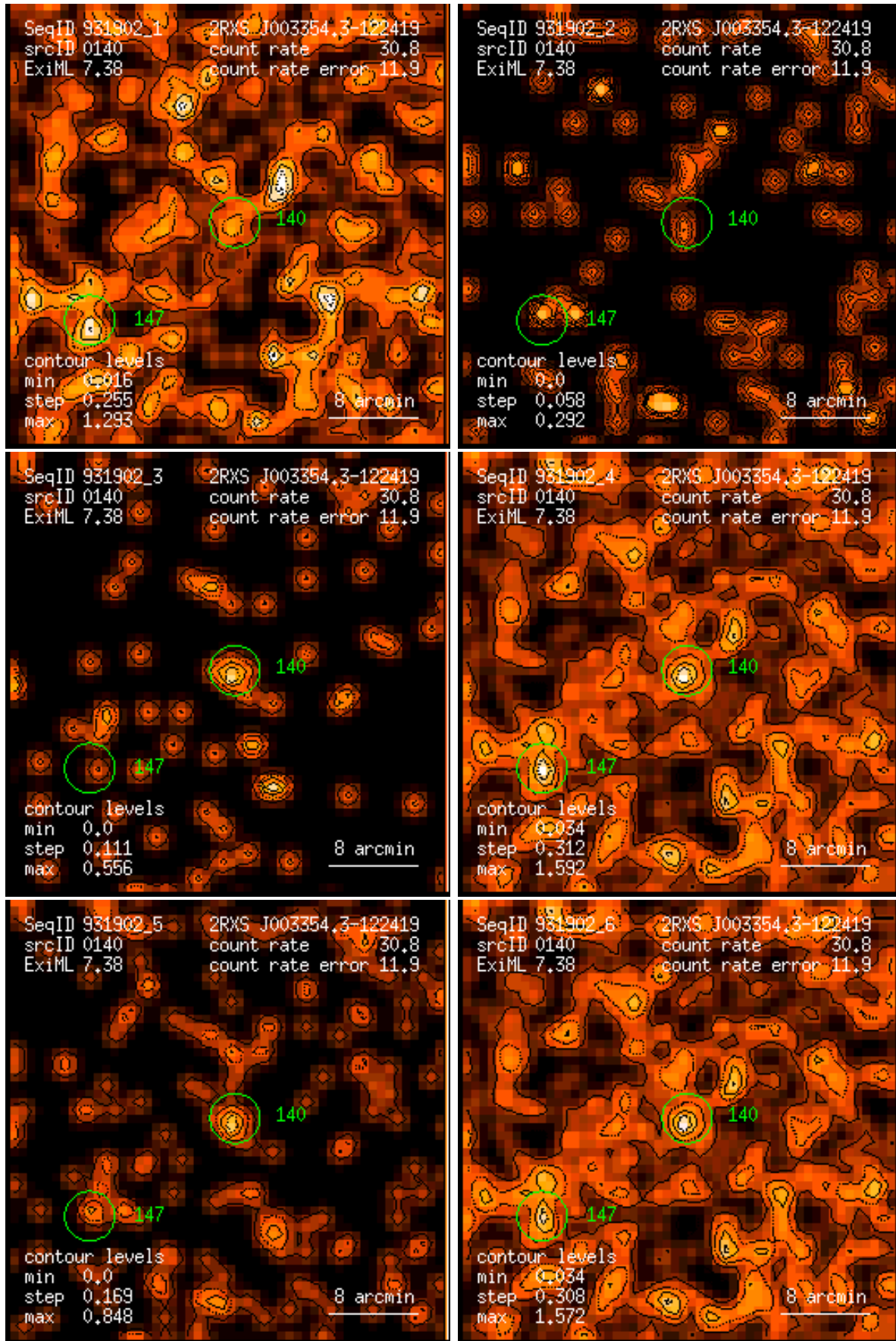
Figure 140: RASS 931902: detection 0140: band rate images, Gaussian filter: (1) PSPC channels 11 – 41, (2) 52 – 90, (3) 91 – 201, (4) 11 – 235, (5) 52 – 201, (6) 11 – 201. Broad band rates in counts/ks. Band rate contour levels in counts/ks/arcmin 2 .
