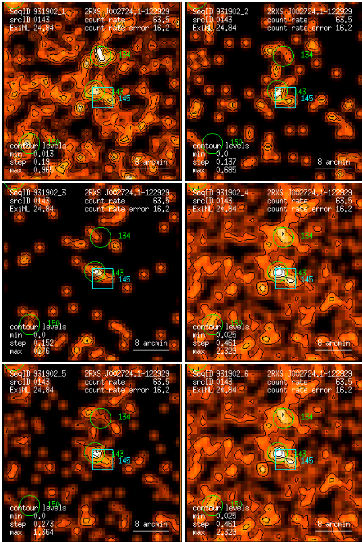
Figure 143: RASS 931902: detection 0143: band rate images, Gaussian filter: (1) PSPC channels 11 – 41, (2) 52 – 90, (3) 91 – 201, (4) 11 – 235, (5) 52 – 201, (6) 11 – 201. Broad band rates in counts/ks. Band rate contour levels in counts/ks/arcmin 2 .
