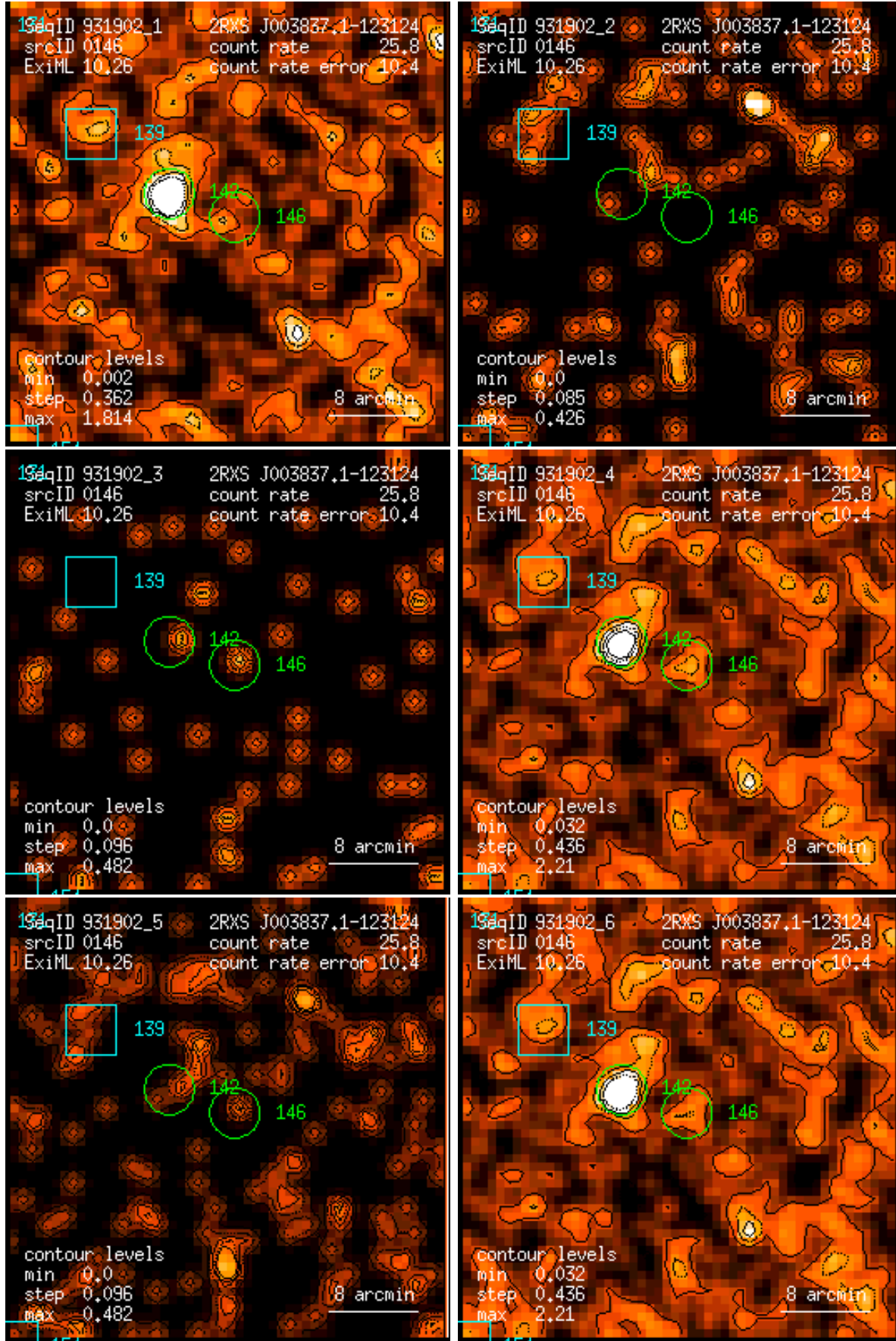
Figure 146: RASS 931902: detection 0146: band rate images, Gaussian filter: (1) PSPC channels 11 – 41, (2) 52 – 90, (3) 91 – 201, (4) 11 – 235, (5) 52 – 201, (6) 11 – 201. Broad band rates in counts/ks. Band rate contour levels in counts/ks/arcmin 2 .
