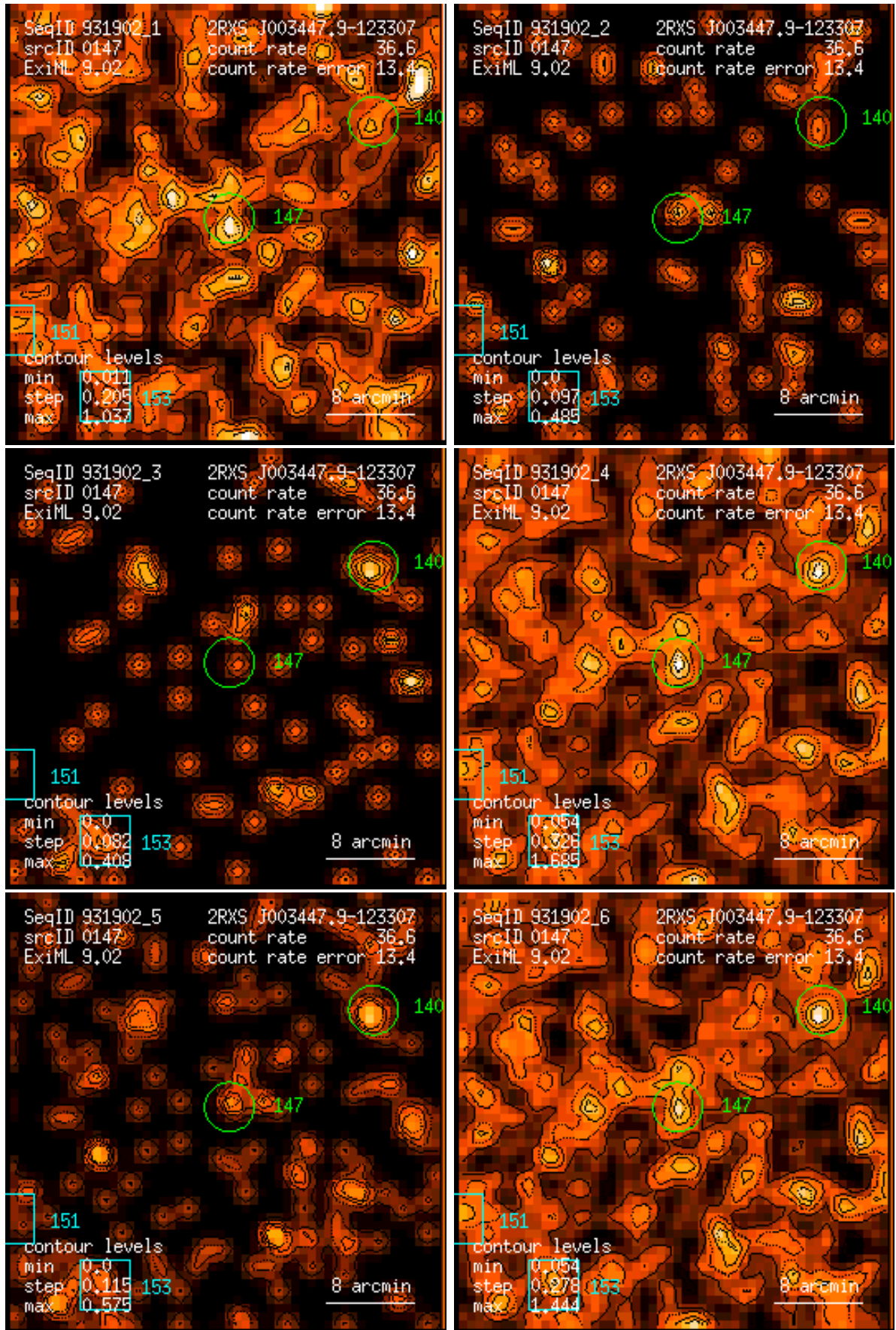
Figure 147: RASS 931902: detection 0147: band rate images, Gaussian filter: (1) PSPC channels 11 – 41, (2) 52 – 90, (3) 91 – 201, (4) 11 – 235, (5) 52 – 201, (6) 11 – 201. Broad band rates in counts/ks. Band rate contour levels in counts/ks/arcmin 2 .
