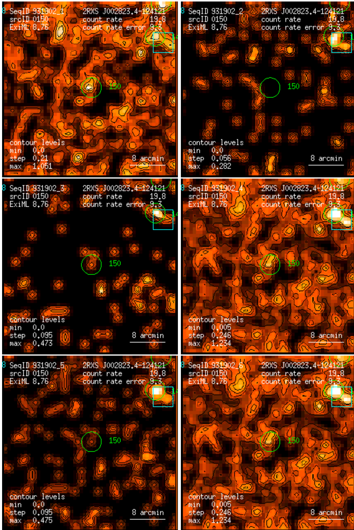
Figure 150: RASS 931902: detection 0150: band rate images, Gaussian filter: (1) PSPC channels 11 – 41, (2) 52 – 90, (3) 91 – 201, (4) 11 – 235, (5) 52 – 201, (6) 11 – 201. Broad band rates in counts/ks. Band rate contour levels in counts/ks/arcmin 2 .
