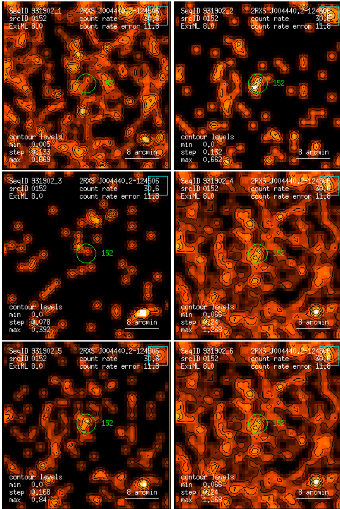
Figure 152: RASS 931902: detection 0152: band rate images, Gaussian filter: (1) PSPC channels 11 – 41, (2) 52 – 90, (3) 91 – 201, (4) 11 – 235, (5) 52 – 201, (6) 11 – 201. Broad band rates in counts/ks. Band rate contour levels in counts/ks/arcmin 2 .
