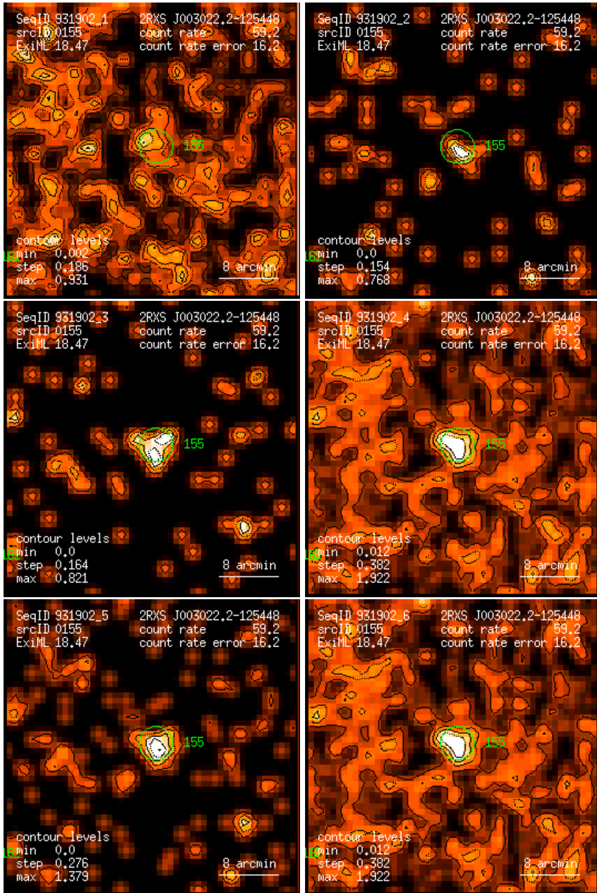
Figure 155: RASS 931902: detection 0155: band rate images, Gaussian filter: (1) PSPC channels 11 – 41, (2) 52 – 90, (3) 91 – 201, (4) 11 – 235, (5) 52 – 201, (6) 11 – 201. Broad band rates in counts/ks. Band rate contour levels in counts/ks/arcmin 2 .
