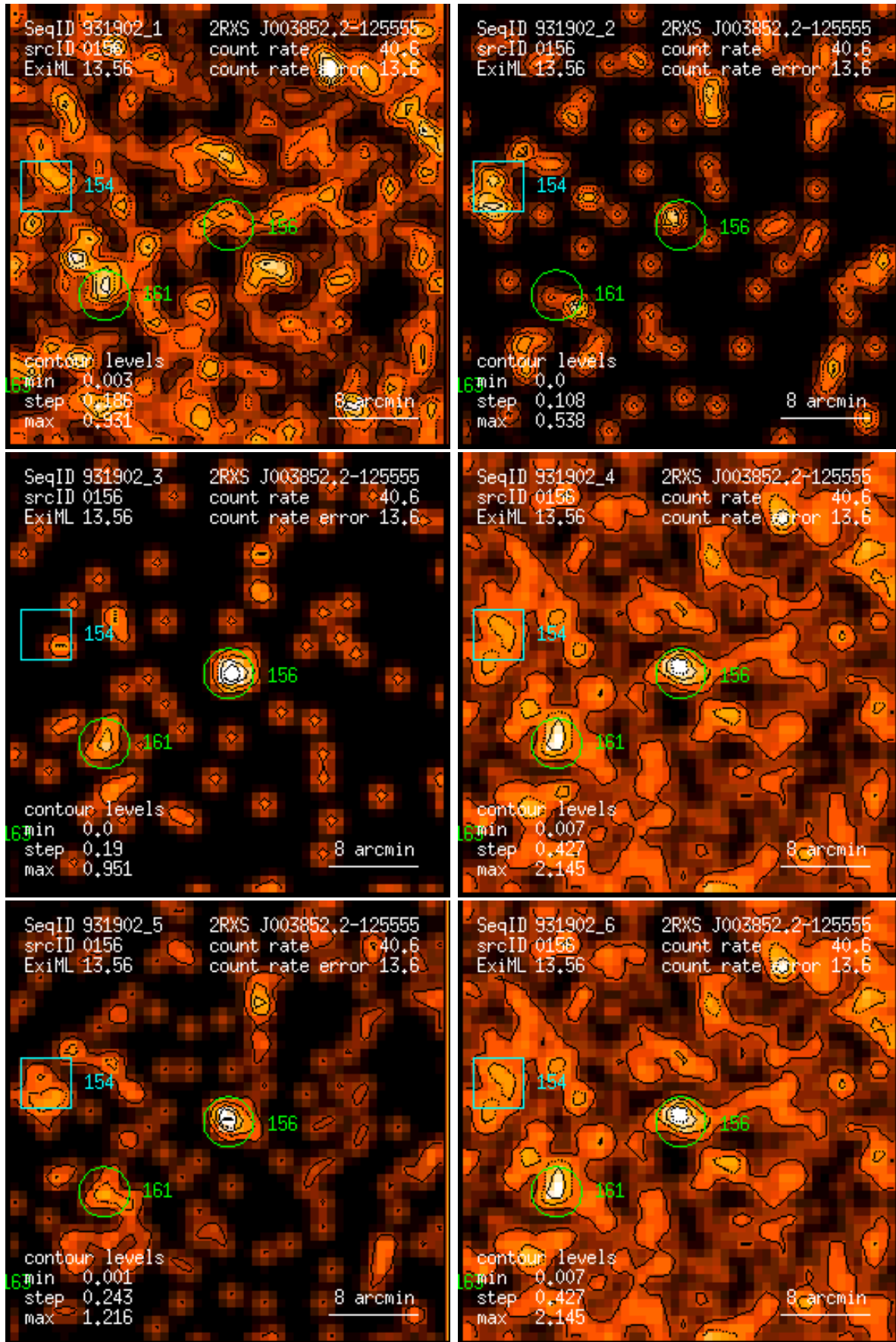
Figure 156: RASS 931902: detection 0156: band rate images, Gaussian filter: (1) PSPC channels 11 – 41, (2) 52 – 90, (3) 91 – 201, (4) 11 – 235, (5) 52 – 201, (6) 11 – 201. Broad band rates in counts/ks. Band rate contour levels in counts/ks/arcmin 2 .
