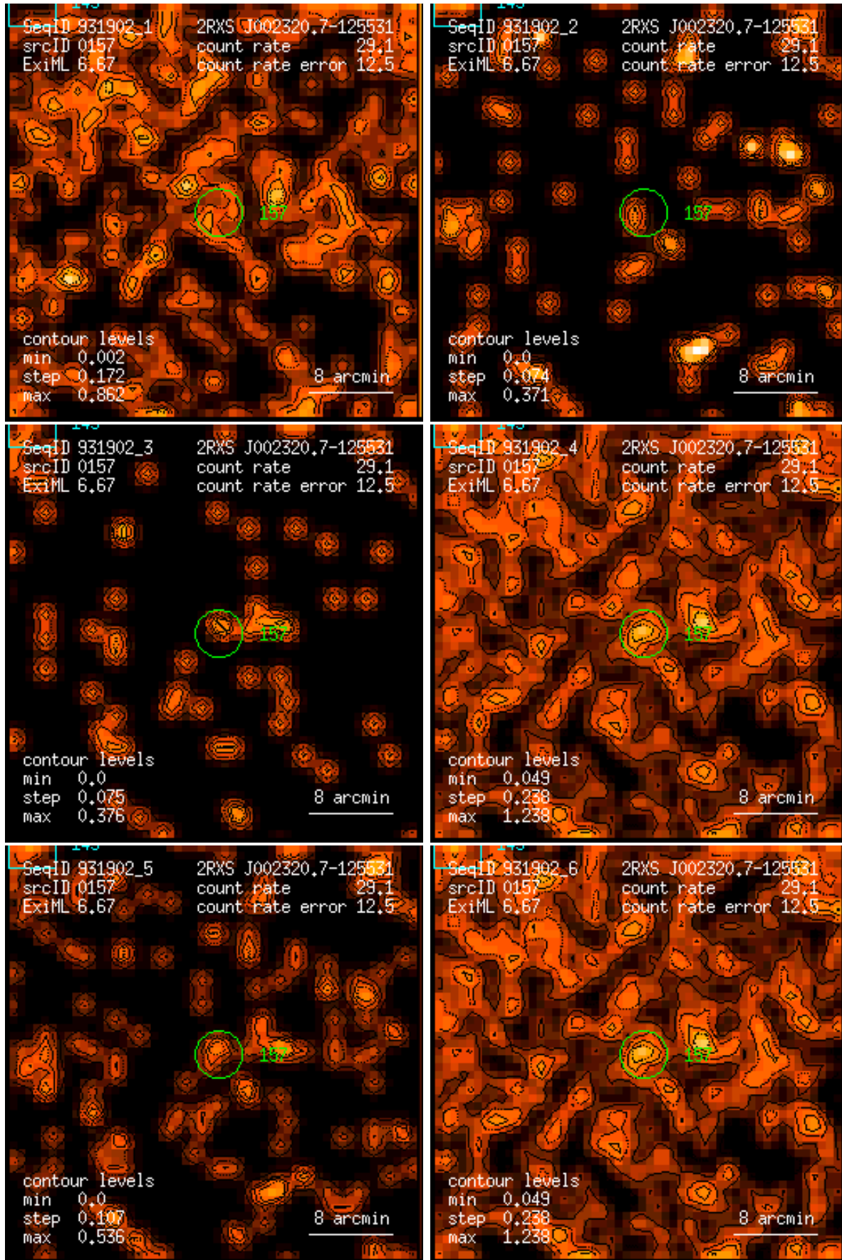
Figure 157: RASS 931902: detection 0157: band rate images, Gaussian filter: (1) PSPC channels 11 – 41, (2) 52 – 90, (3) 91 – 201, (4) 11 – 235, (5) 52 – 201, (6) 11 – 201. Broad band rates in counts/ks. Band rate contour levels in counts/ks/arcmin 2 .
