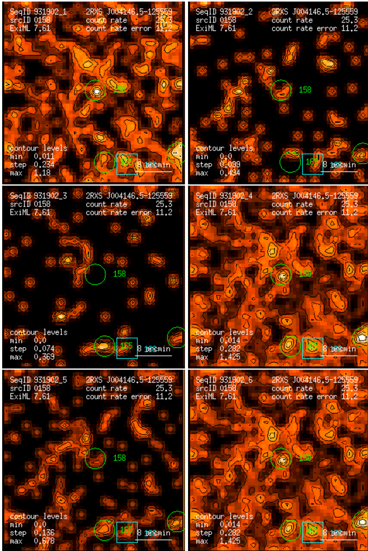
Figure 158: RASS 931902: detection 0158: band rate images, Gaussian filter: (1) PSPC channels 11 – 41, (2) 52 – 90, (3) 91 – 201, (4) 11 – 235, (5) 52 – 201, (6) 11 – 201. Broad band rates in counts/ks. Band rate contour levels in counts/ks/arcmin 2 .
