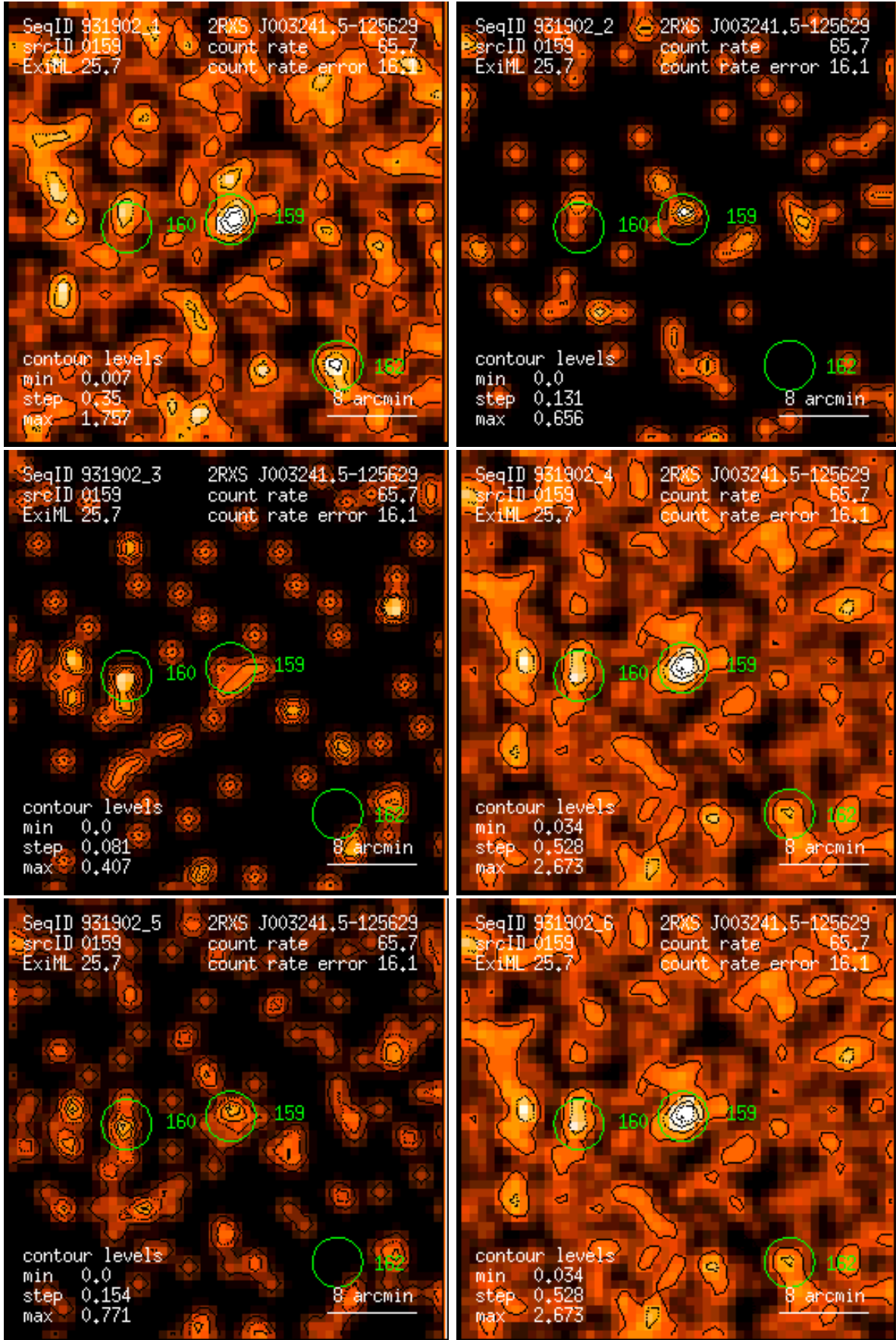
Figure 159: RASS 931902: detection 0159: band rate images, Gaussian filter: (1) PSPC channels 11 – 41, (2) 52 – 90, (3) 91 – 201, (4) 11 – 235, (5) 52 – 201, (6) 11 – 201. Broad band rates in counts/ks. Band rate contour levels in counts/ks/arcmin 2 .
