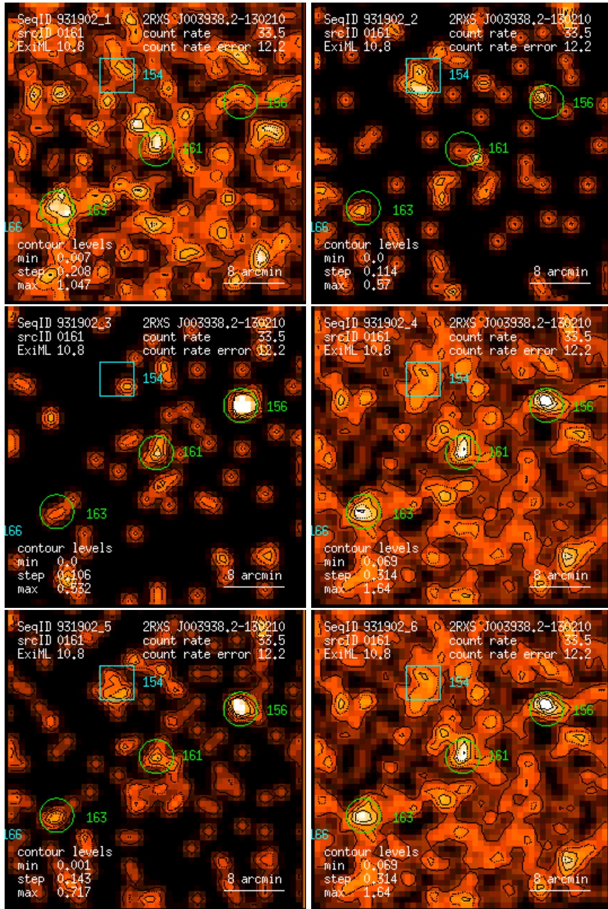
Figure 161: RASS 931902: detection 0161: band rate images, Gaussian filter: (1) PSPC channels 11 – 41, (2) 52 – 90, (3) 91 – 201, (4) 11 – 235, (5) 52 – 201, (6) 11 – 201. Broad band rates in counts/ks. Band rate contour levels in counts/ks/arcmin 2 .
