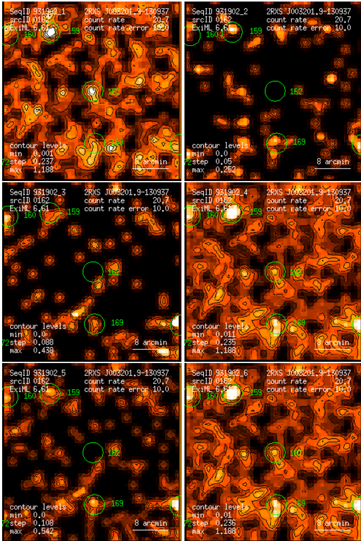
Figure 162: RASS 931902: detection 0162: band rate images, Gaussian filter: (1) PSPC channels 11 – 41, (2) 52 – 90, (3) 91 – 201, (4) 11 – 235, (5) 52 – 201, (6) 11 – 201. Broad band rates in counts/ks. Band rate contour levels in counts/ks/arcmin 2 .
