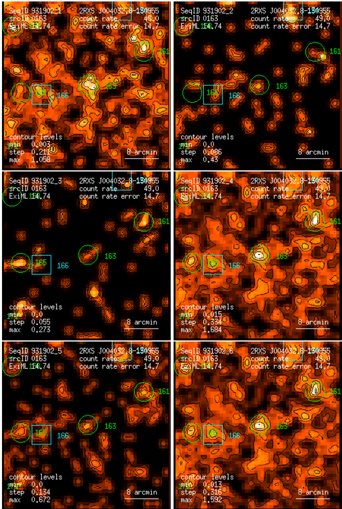
Figure 163: RASS 931902: detection 0163: band rate images, Gaussian filter: (1) PSPC channels 11 – 41, (2) 52 – 90, (3) 91 – 201, (4) 11 – 235, (5) 52 – 201, (6) 11 – 201. Broad band rates in counts/ks. Band rate contour levels in counts/ks/arcmin 2 .
