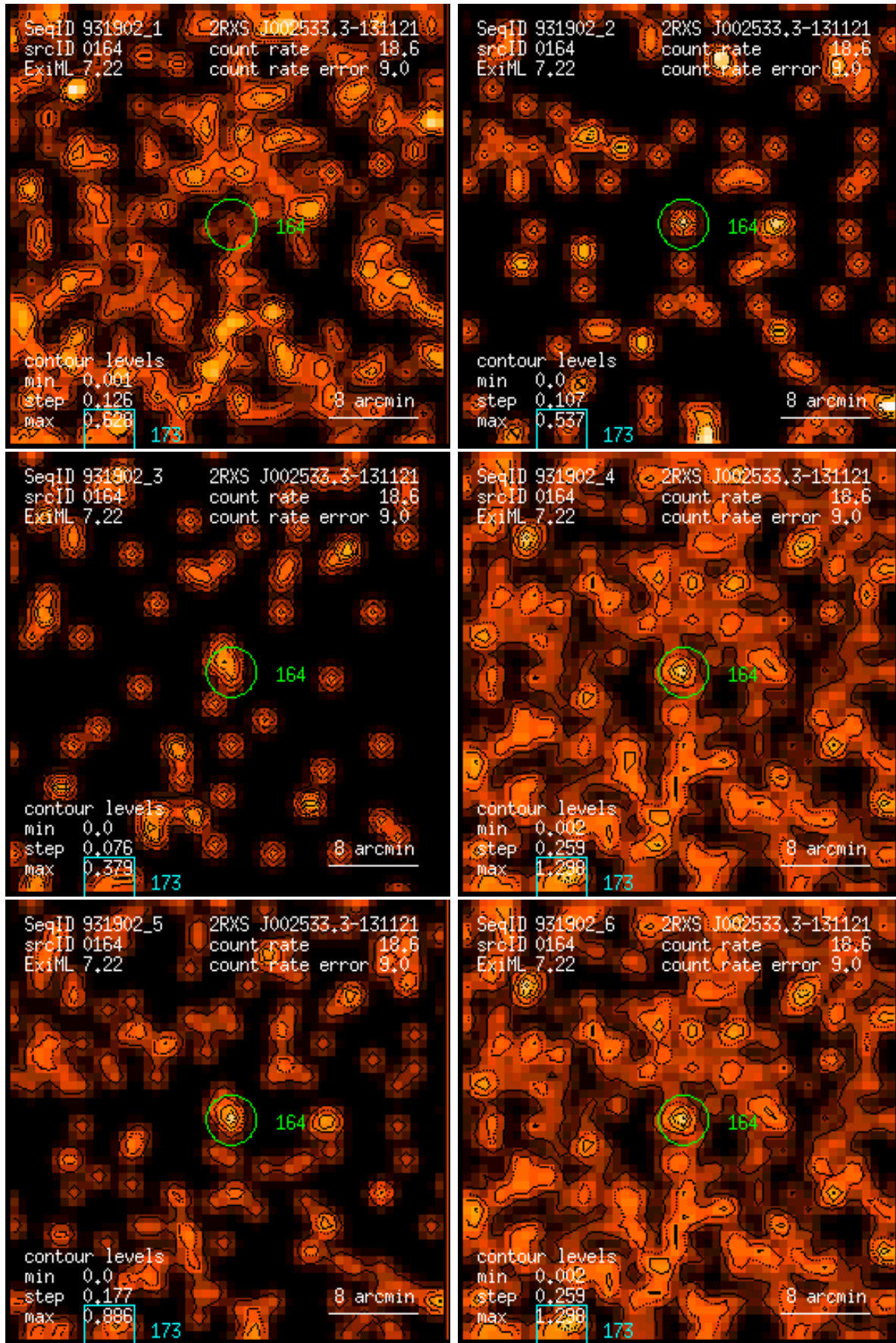
Figure 164: RASS 931902: detection 0164: band rate images, Gaussian filter: (1) PSPC channels 11 – 41, (2) 52 – 90, (3) 91 – 201, (4) 11 – 235, (5) 52 – 201, (6) 11 – 201. Broad band rates in counts/ks. Band rate contour levels in counts/ks/arcmin 2 .
