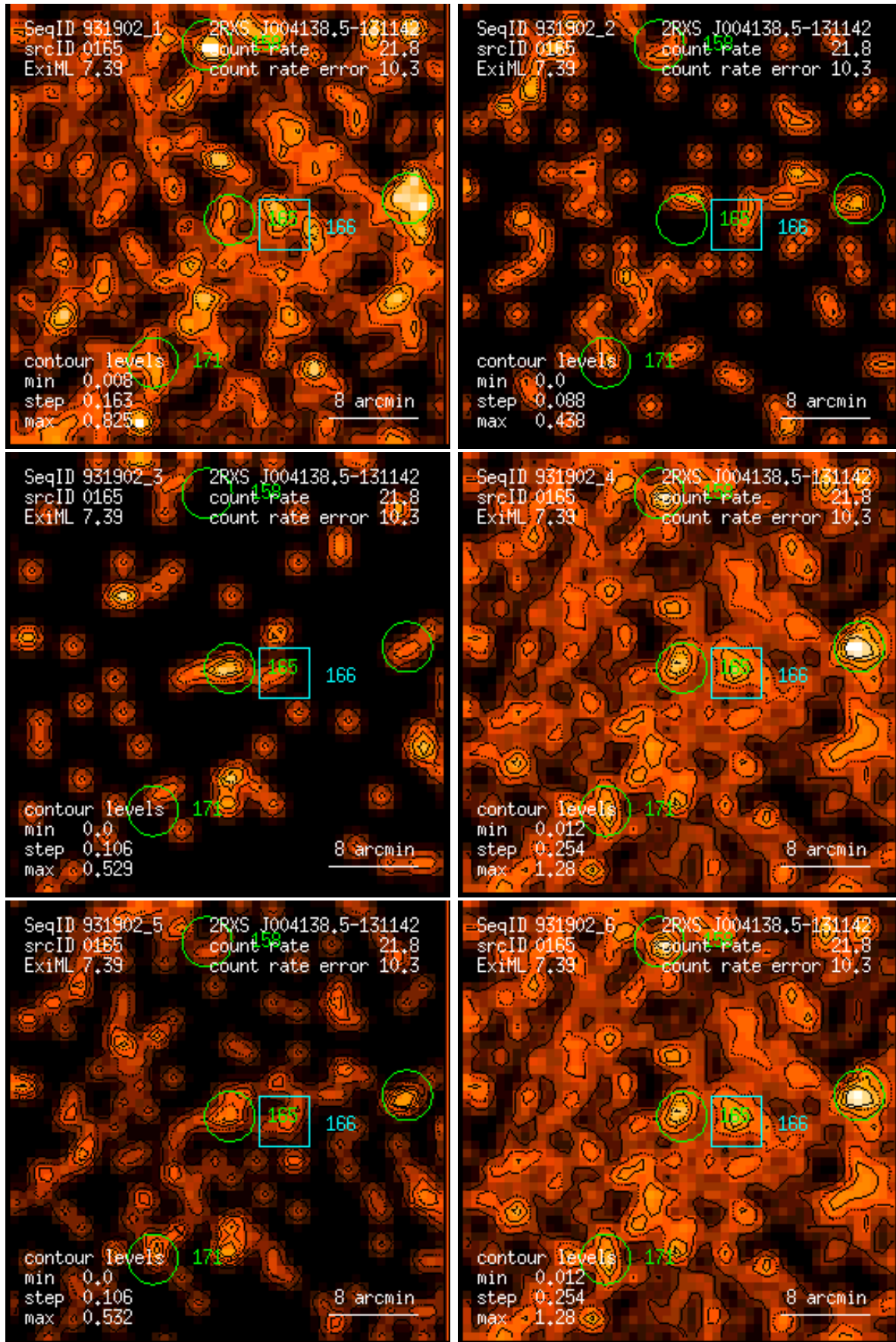
Figure 165: RASS 931902: detection 0165: band rate images, Gaussian filter: (1) PSPC channels 11 – 41, (2) 52 – 90, (3) 91 – 201, (4) 11 – 235, (5) 52 – 201, (6) 11 – 201. Broad band rates in counts/ks. Band rate contour levels in counts/ks/arcmin 2 .
