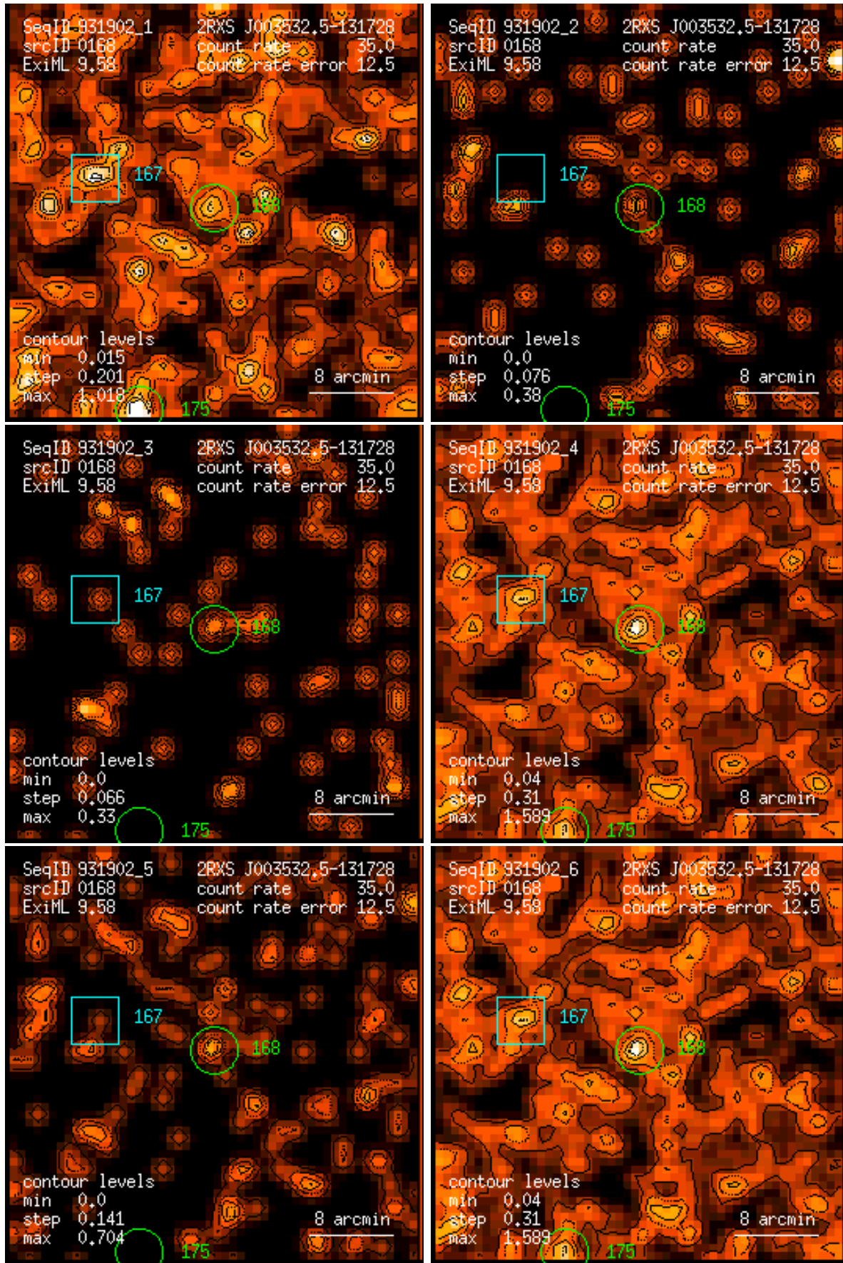
Figure 168: RASS 931902: detection 0168: band rate images, Gaussian filter: (1) PSPC channels 11 – 41, (2) 52 – 90, (3) 91 – 201, (4) 11 – 235, (5) 52 – 201, (6) 11 – 201. Broad band rates in counts/ks. Band rate contour levels in counts/ks/arcmin 2 .
