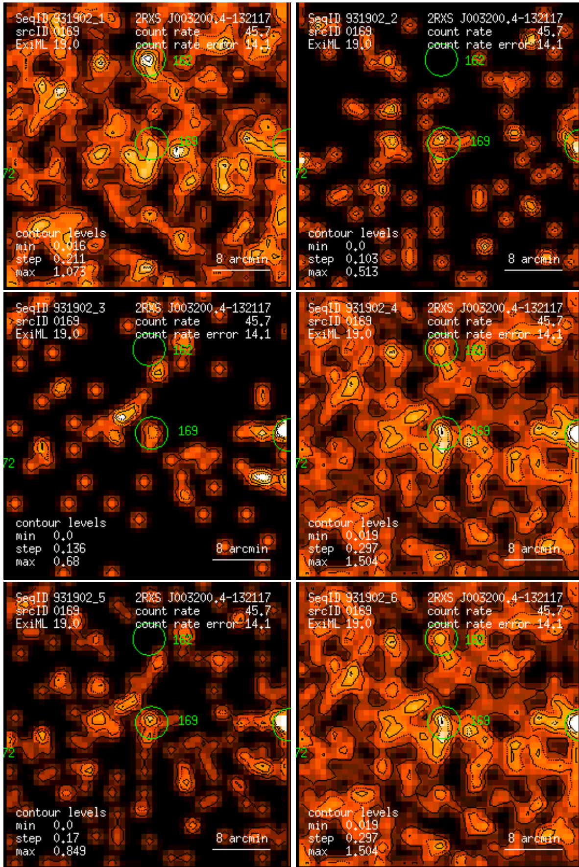
Figure 169: RASS 931902: detection 0169: band rate images, Gaussian filter: (1) PSPC channels 11 – 41, (2) 52 – 90, (3) 91 – 201, (4) 11 – 235, (5) 52 – 201, (6) 11 – 201. Broad band rates in counts/ks. Band rate contour levels in counts/ks/arcmin 2 .
