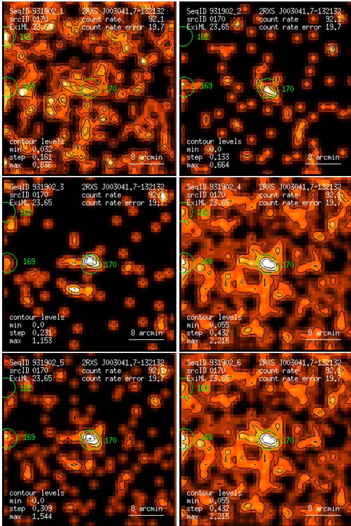
Figure 170: RASS 931902: detection 0170: band rate images, Gaussian filter: (1) PSPC channels 11 – 41, (2) 52 – 90, (3) 91 – 201, (4) 11 – 235, (5) 52 – 201, (6) 11 – 201. Broad band rates in counts/ks. Band rate contour levels in counts/ks/arcmin 2 .
