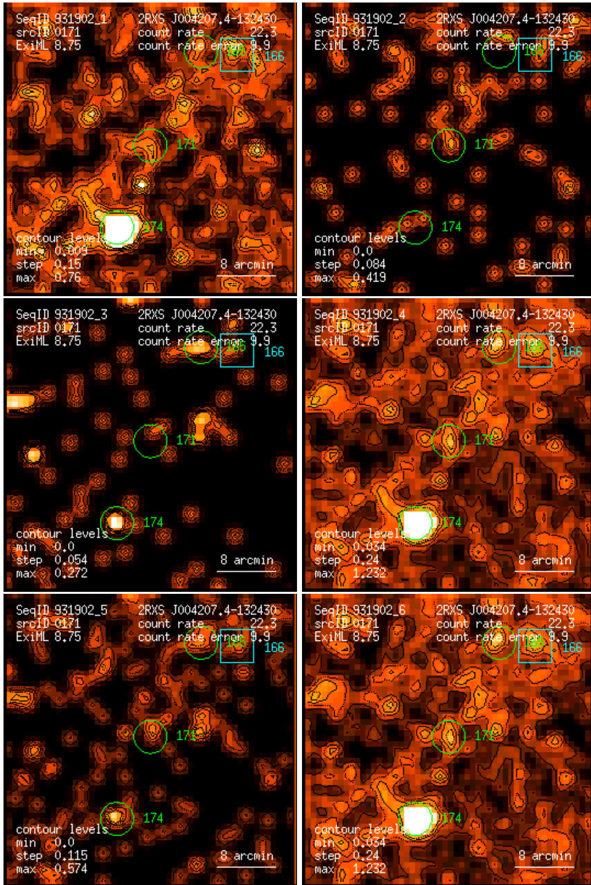
Figure 171: RASS 931902: detection 0171: band rate images, Gaussian filter: (1) PSPC channels 11 – 41, (2) 52 – 90, (3) 91 – 201, (4) 11 – 235, (5) 52 – 201, (6) 11 – 201. Broad band rates in counts/ks. Band rate contour levels in counts/ks/arcmin 2 .
