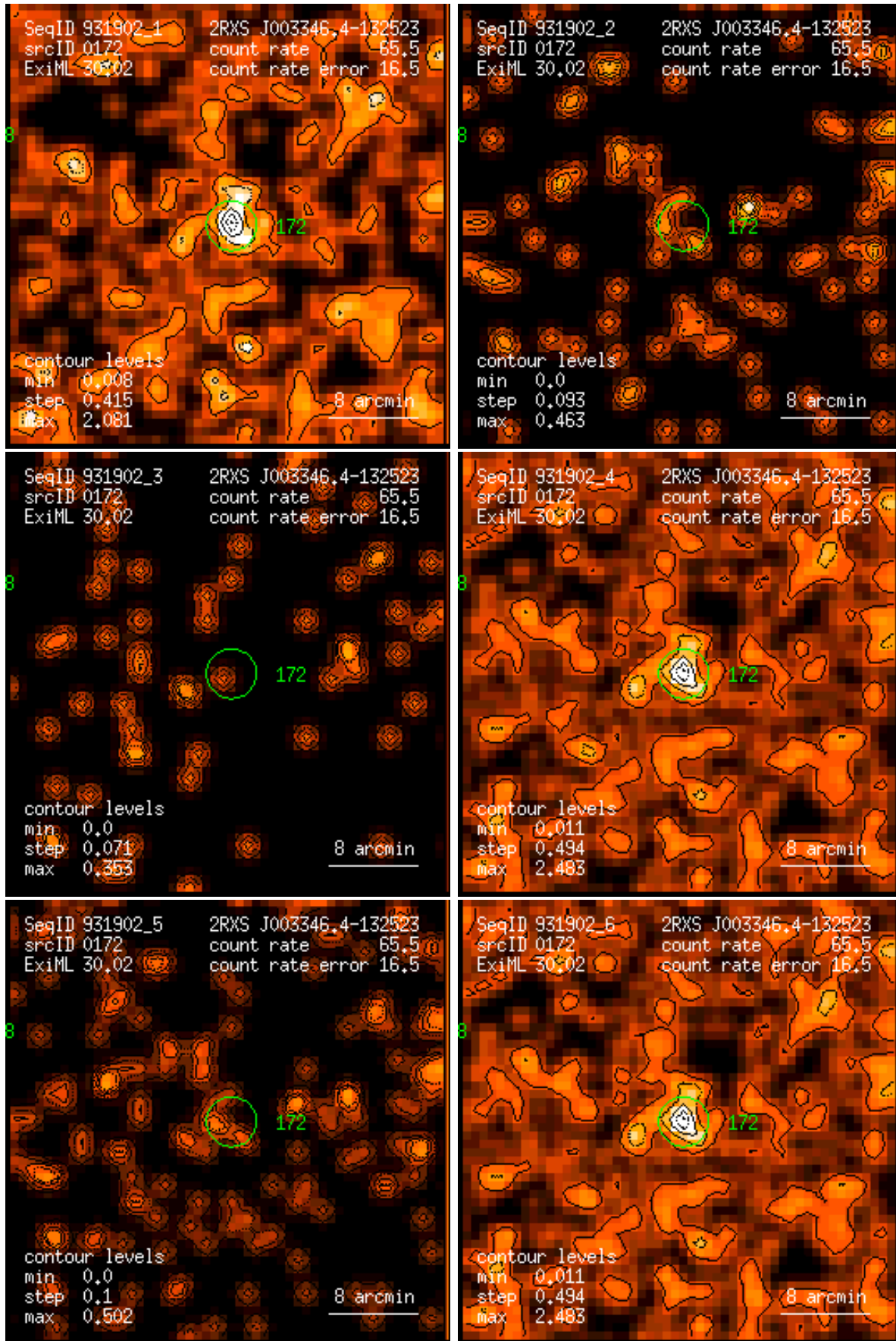
Figure 172: RASS 931902: detection 0172: band rate images, Gaussian filter: (1) PSPC channels 11 – 41, (2) 52 – 90, (3) 91 – 201, (4) 11 – 235, (5) 52 – 201, (6) 11 – 201. Broad band rates in counts/ks. Band rate contour levels in counts/ks/arcmin 2 .
