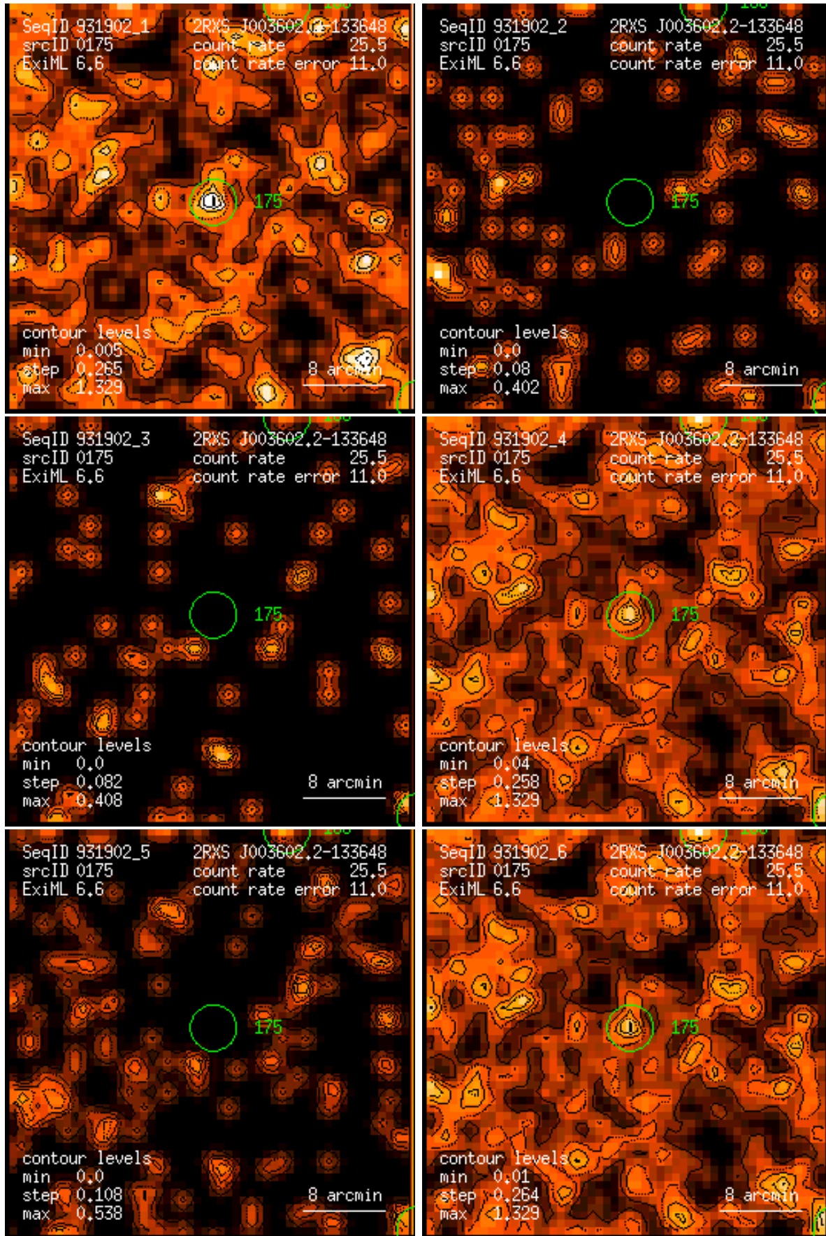
Figure 175: RASS 931902: detection 0175: band rate images, Gaussian filter: (1) PSPC channels 11 – 41, (2) 52 – 90, (3) 91 – 201, (4) 11 – 235, (5) 52 – 201, (6) 11 – 201. Broad band rates in counts/ks. Band rate contour levels in counts/ks/arcmin 2 .
