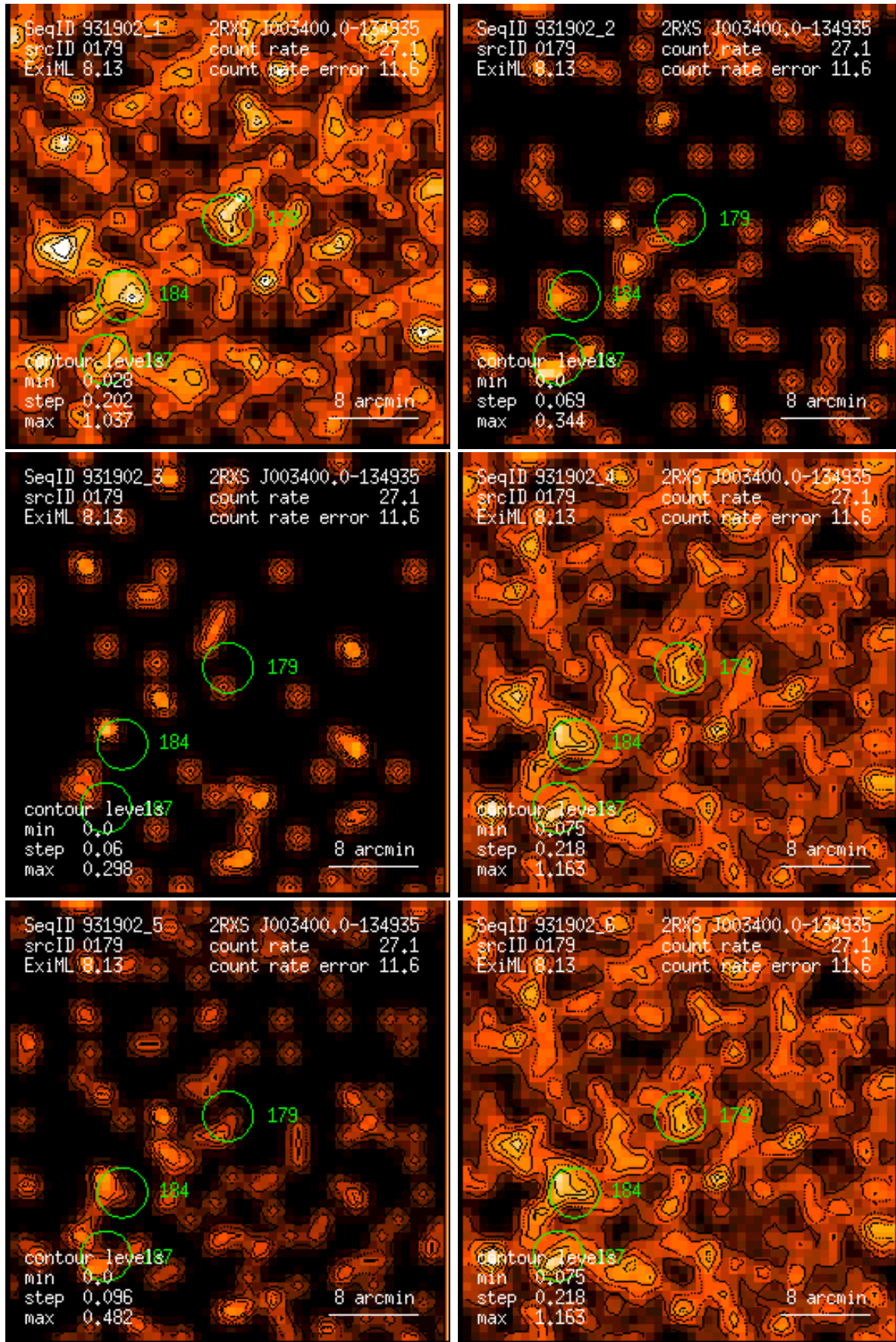
Figure 179: RASS 931902: detection 0179: band rate images, Gaussian filter: (1) PSPC channels 11 – 41, (2) 52 – 90, (3) 91 – 201, (4) 11 – 235, (5) 52 – 201, (6) 11 – 201. Broad band rates in counts/ks. Band rate contour levels in counts/ks/arcmin 2 .
