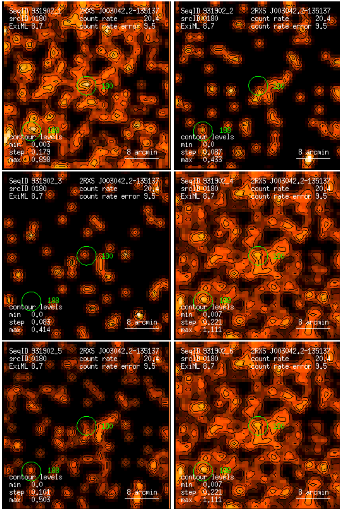
Figure 180: RASS 931902: detection 0180: band rate images, Gaussian filter: (1) PSPC channels 11 – 41, (2) 52 – 90, (3) 91 – 201, (4) 11 – 235, (5) 52 – 201, (6) 11 – 201. Broad band rates in counts/ks. Band rate contour levels in counts/ks/arcmin 2 .
