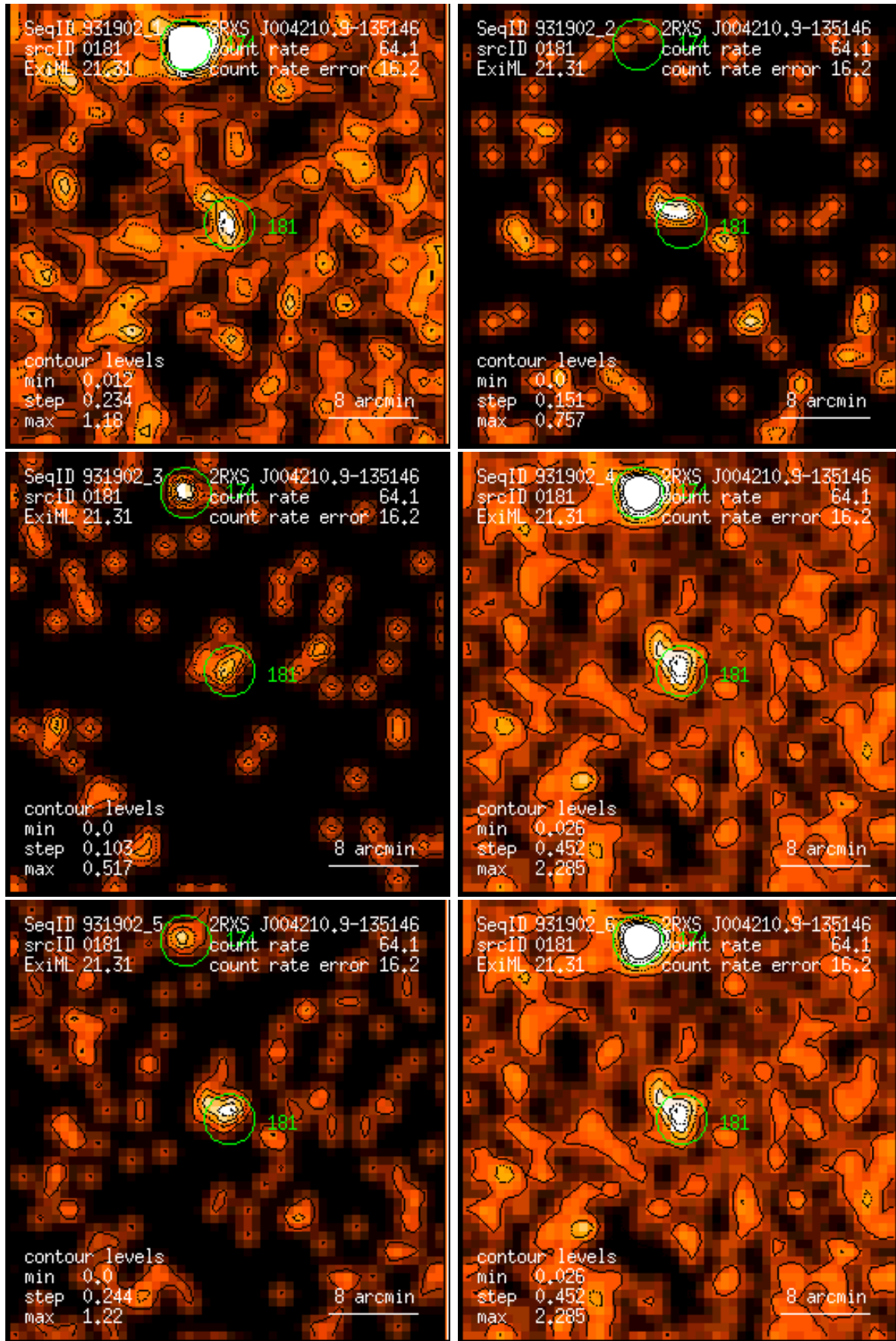
Figure 181: RASS 931902: detection 0181: band rate images, Gaussian filter: (1) PSPC channels 11 – 41, (2) 52 – 90, (3) 91 – 201, (4) 11 – 235, (5) 52 – 201, (6) 11 – 201. Broad band rates in counts/ks. Band rate contour levels in counts/ks/arcmin 2 .
