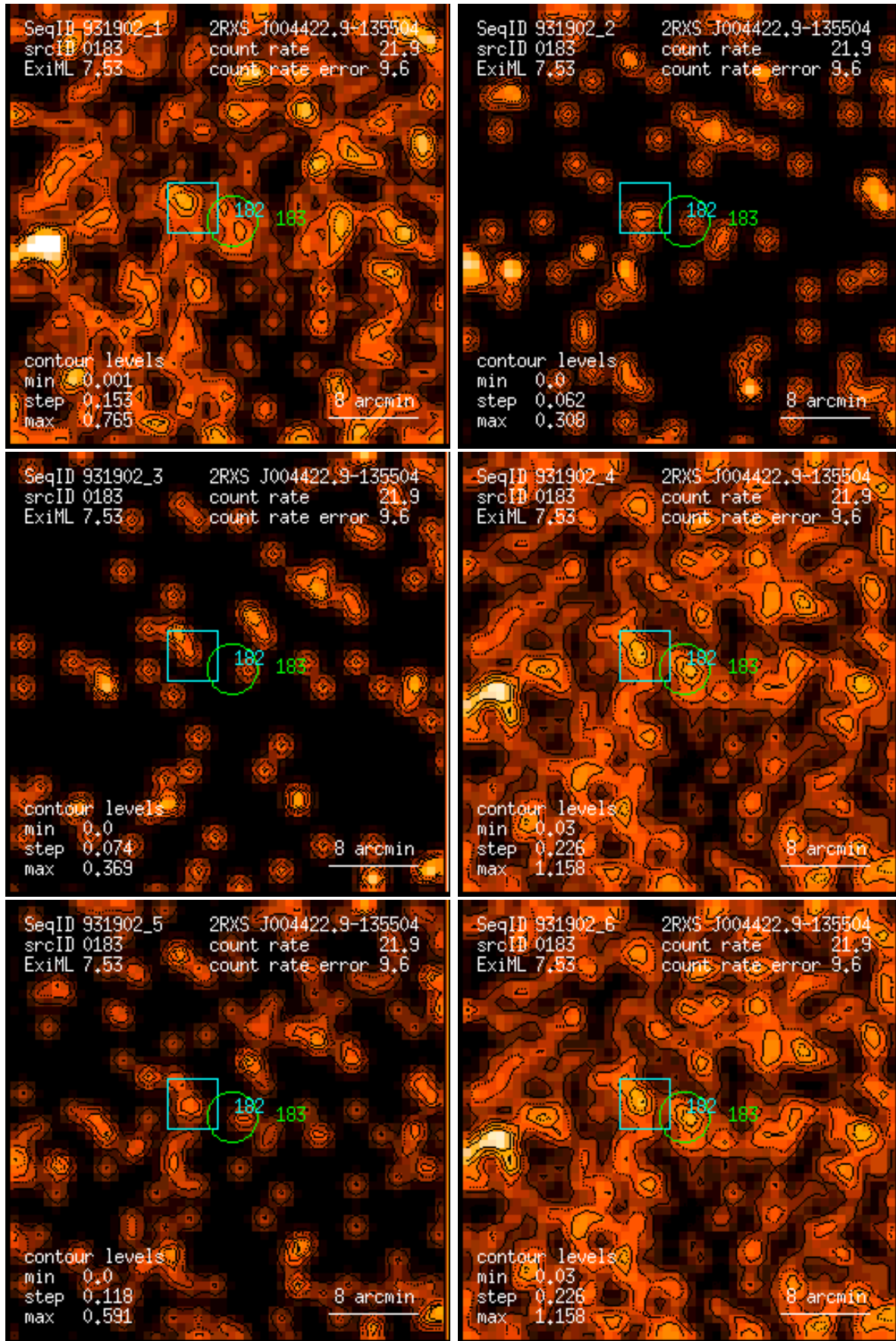
Figure 183: RASS 931902: detection 0183: band rate images, Gaussian filter: (1) PSPC channels 11 – 41, (2) 52 – 90, (3) 91 – 201, (4) 11 – 235, (5) 52 – 201, (6) 11 – 201. Broad band rates in counts/ks. Band rate contour levels in counts/ks/arcmin 2 .
