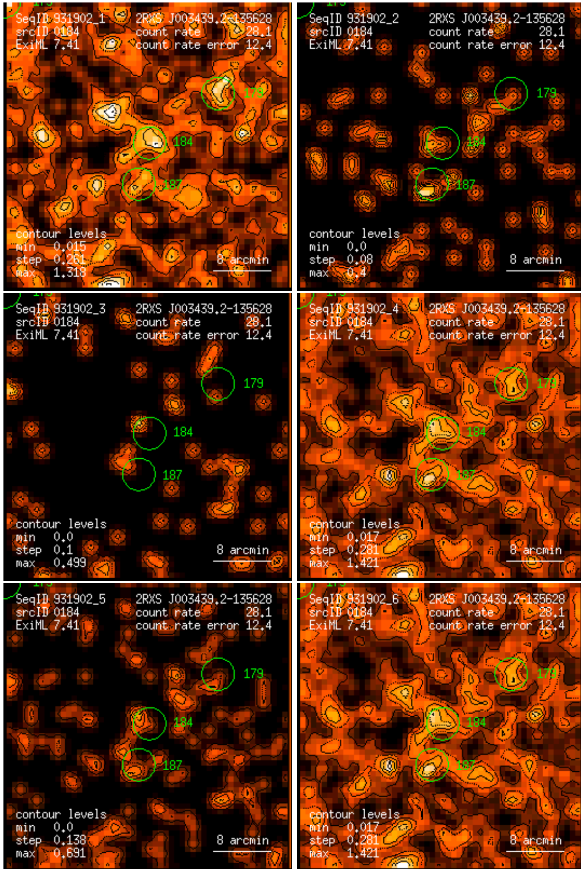
Figure 184: RASS 931902: detection 0184: band rate images, Gaussian filter: (1) PSPC channels 11 – 41, (2) 52 – 90, (3) 91 – 201, (4) 11 – 235, (5) 52 – 201, (6) 11 – 201. Broad band rates in counts/ks. Band rate contour levels in counts/ks/arcmin 2 .
