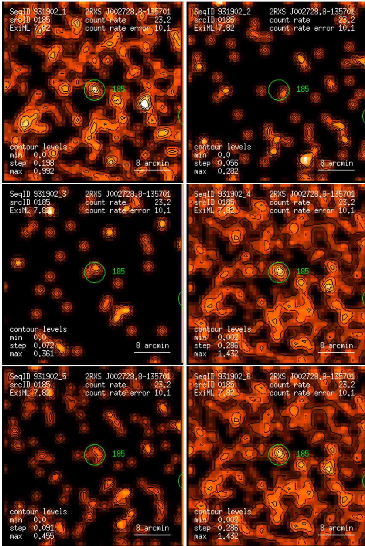
Figure 185: RASS 931902: detection 0185: band rate images, Gaussian filter: (1) PSPC channels 11 – 41, (2) 52 – 90, (3) 91 – 201, (4) 11 – 235, (5) 52 – 201, (6) 11 – 201. Broad band rates in counts/ks. Band rate contour levels in counts/ks/arcmin 2 .
