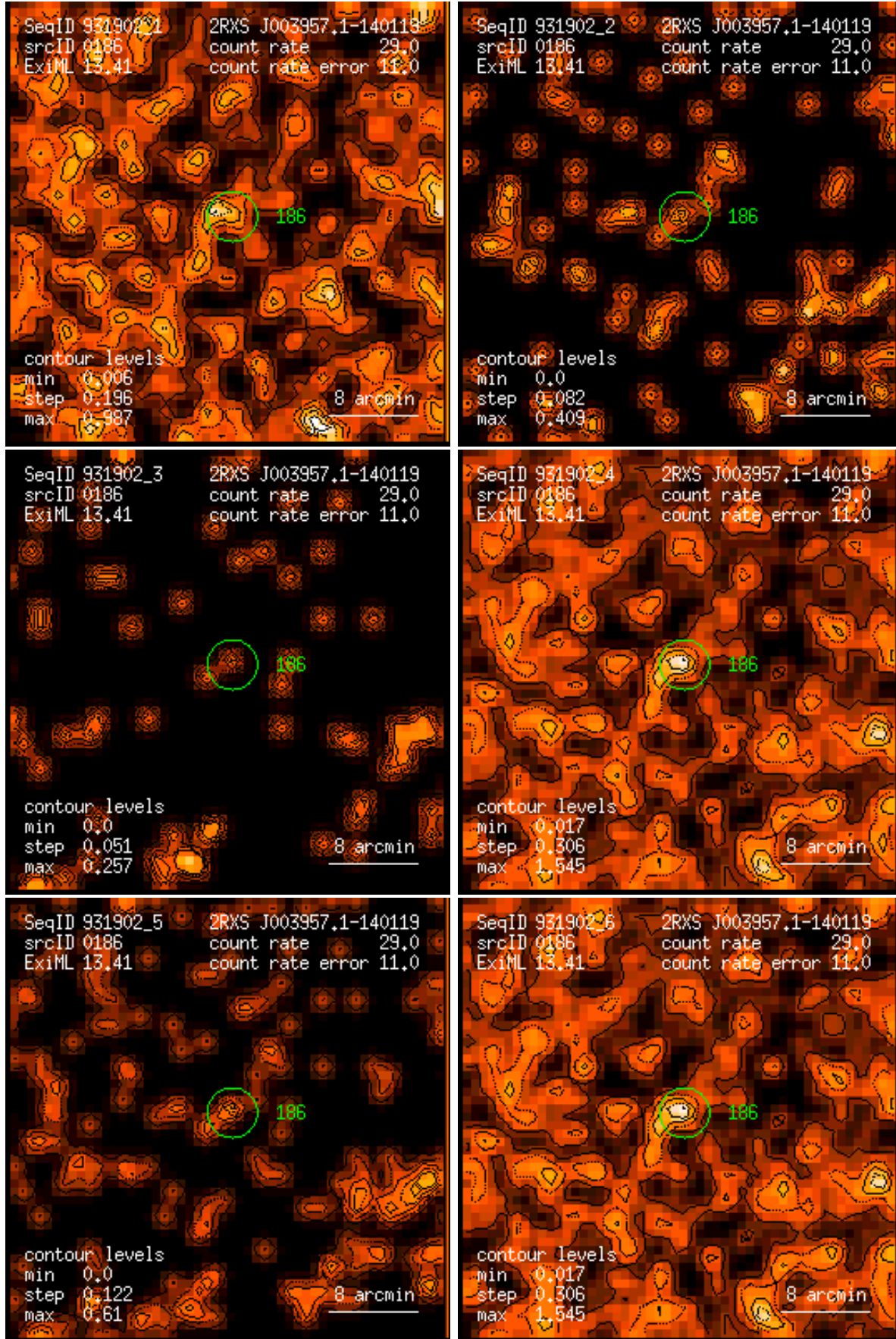
Figure 186: RASS 931902: detection 0186: band rate images, Gaussian filter: (1) PSPC channels 11 – 41, (2) 52 – 90, (3) 91 – 201, (4) 11 – 235, (5) 52 – 201, (6) 11 – 201. Broad band rates in counts/ks. Band rate contour levels in counts/ks/arcmin 2 .
