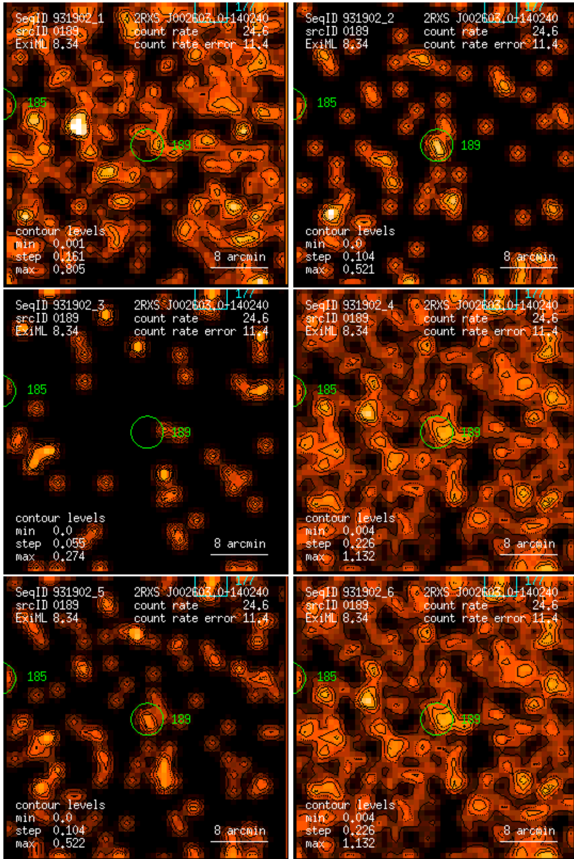
Figure 189: RASS 931902: detection 0189: band rate images, Gaussian filter: (1) PSPC channels 11 – 41, (2) 52 – 90, (3) 91 – 201, (4) 11 – 235, (5) 52 – 201, (6) 11 – 201. Broad band rates in counts/ks. Band rate contour levels in counts/ks/arcmin 2 .
