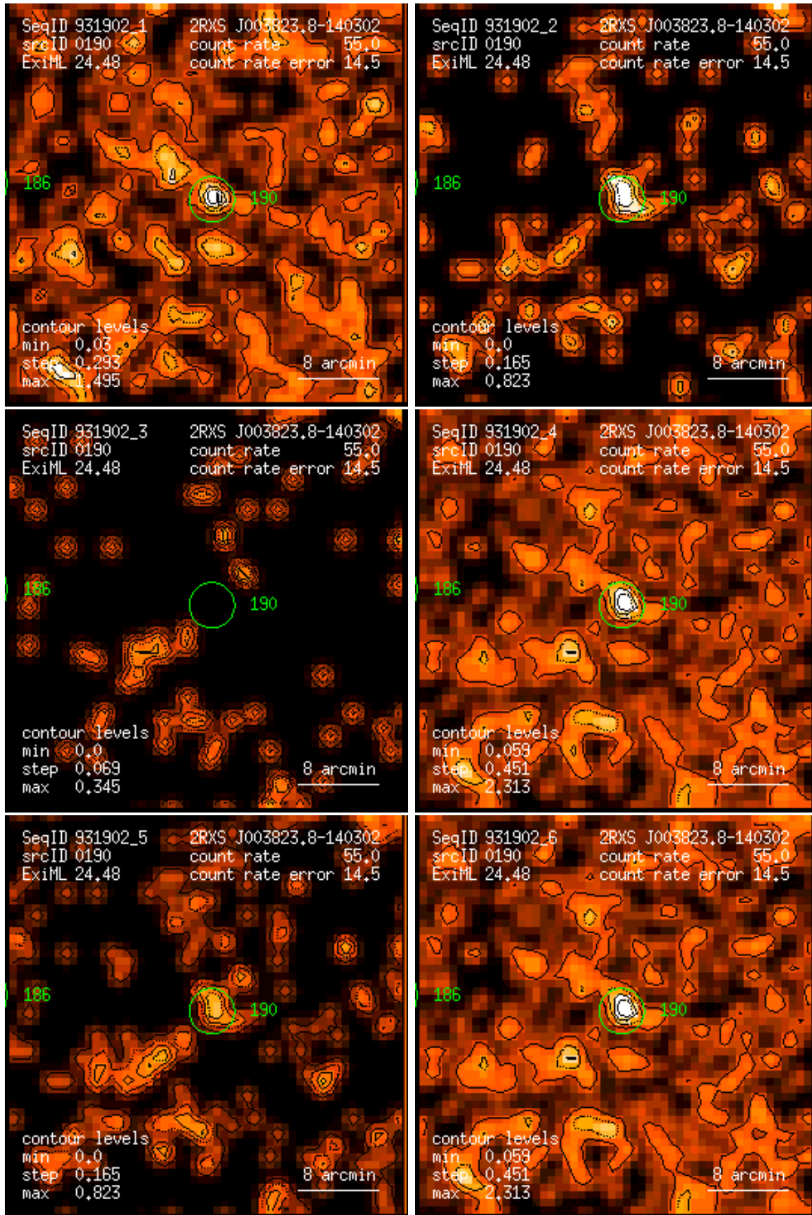
Figure 190: RASS 931902: detection 0190: band rate images, Gaussian filter: (1) PSPC channels 11 – 41, (2) 52 – 90, (3) 91 – 201, (4) 11 – 235, (5) 52 – 201, (6) 11 – 201. Broad band rates in counts/ks. Band rate contour levels in counts/ks/arcmin 2 .
