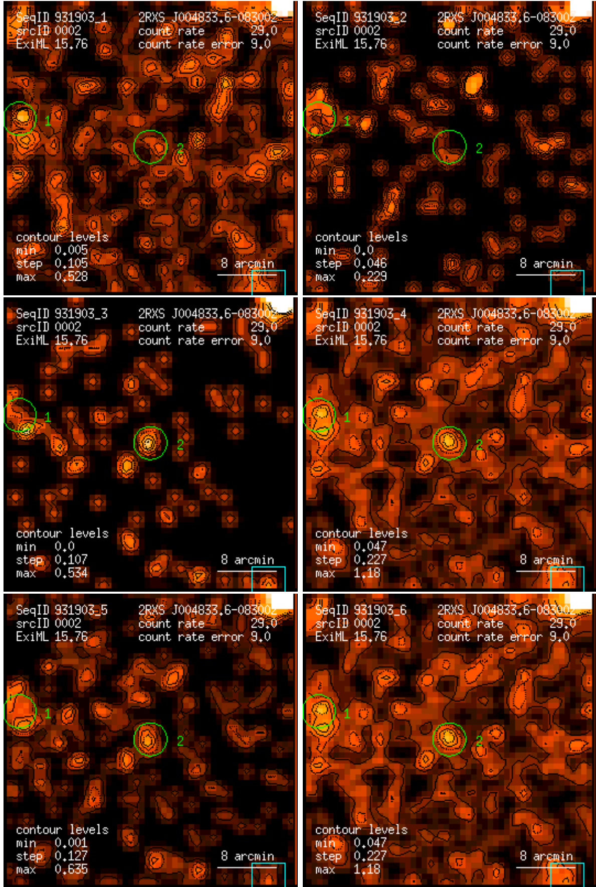
Figure 2: RASS 931903: detection 0002: band rate images, Gaussian filter: (1) PSPC channels 11 – 41, (2) 52 – 90, (3) 91 – 201, (4) 11 – 235, (5) 52 – 201, (6) 11 – 201. Broad band rates in counts/ks. Band rate contour levels in counts/ks/arcmin 2 .
