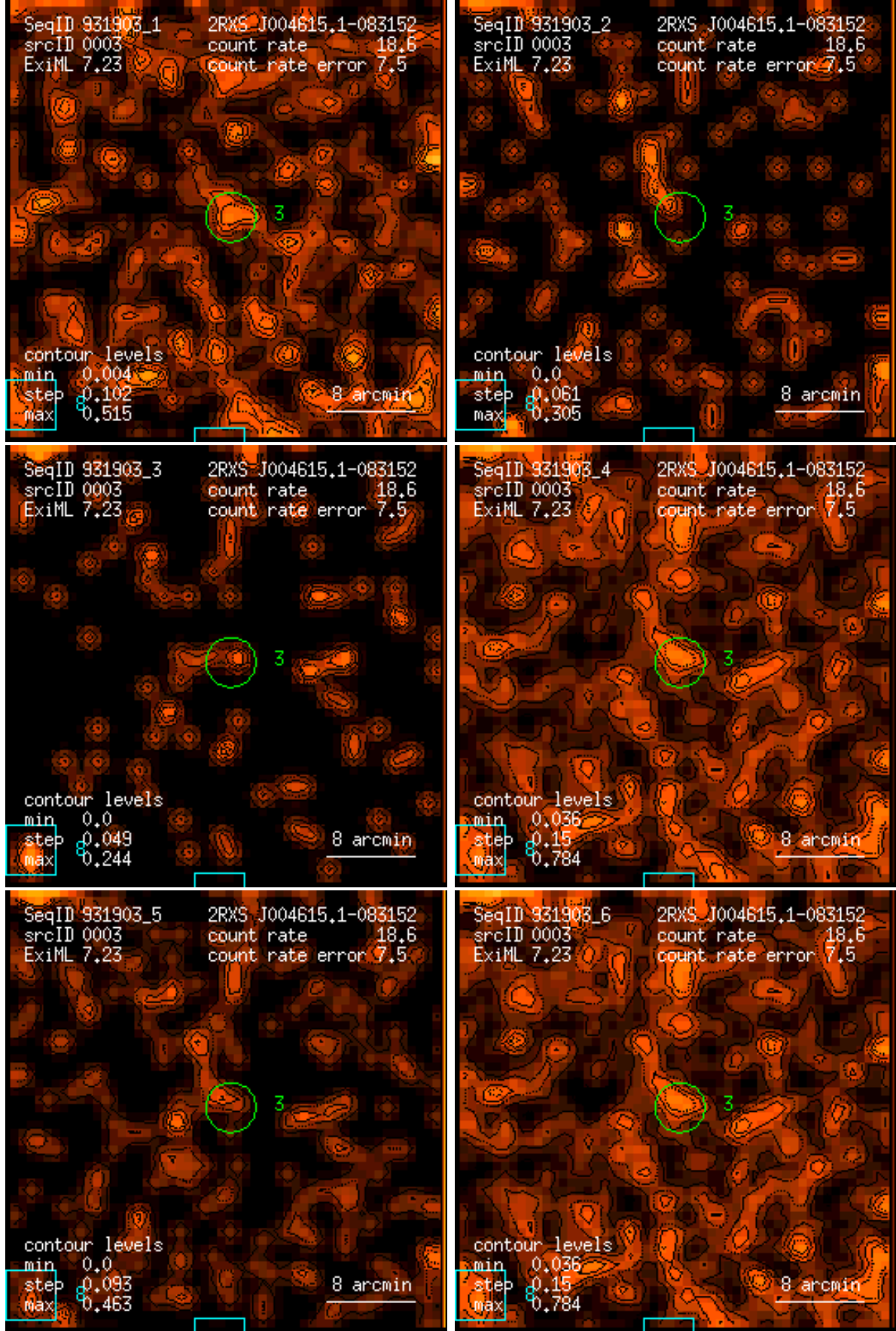
Figure 3: RASS 931903: detection 0003: band rate images, Gaussian filter: (1) PSPC channels 11 – 41, (2) 52 – 90, (3) 91 – 201, (4) 11 – 235, (5) 52 – 201, (6) 11 – 201. Broad band rates in counts/ks. Band rate contour levels in counts/ks/arcmin 2 .
