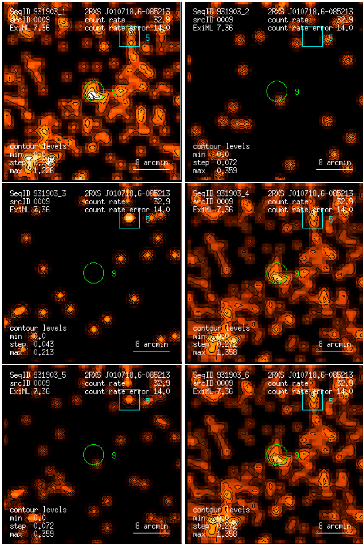
Figure 9: RASS 931903: detection 0009: band rate images, Gaussian filter: (1) PSPC channels 11 – 41, (2) 52 – 90, (3) 91 – 201, (4) 11 – 235, (5) 52 – 201, (6) 11 – 201. Broad band rates in counts/ks. Band rate contour levels in counts/ks/arcmin 2 .
