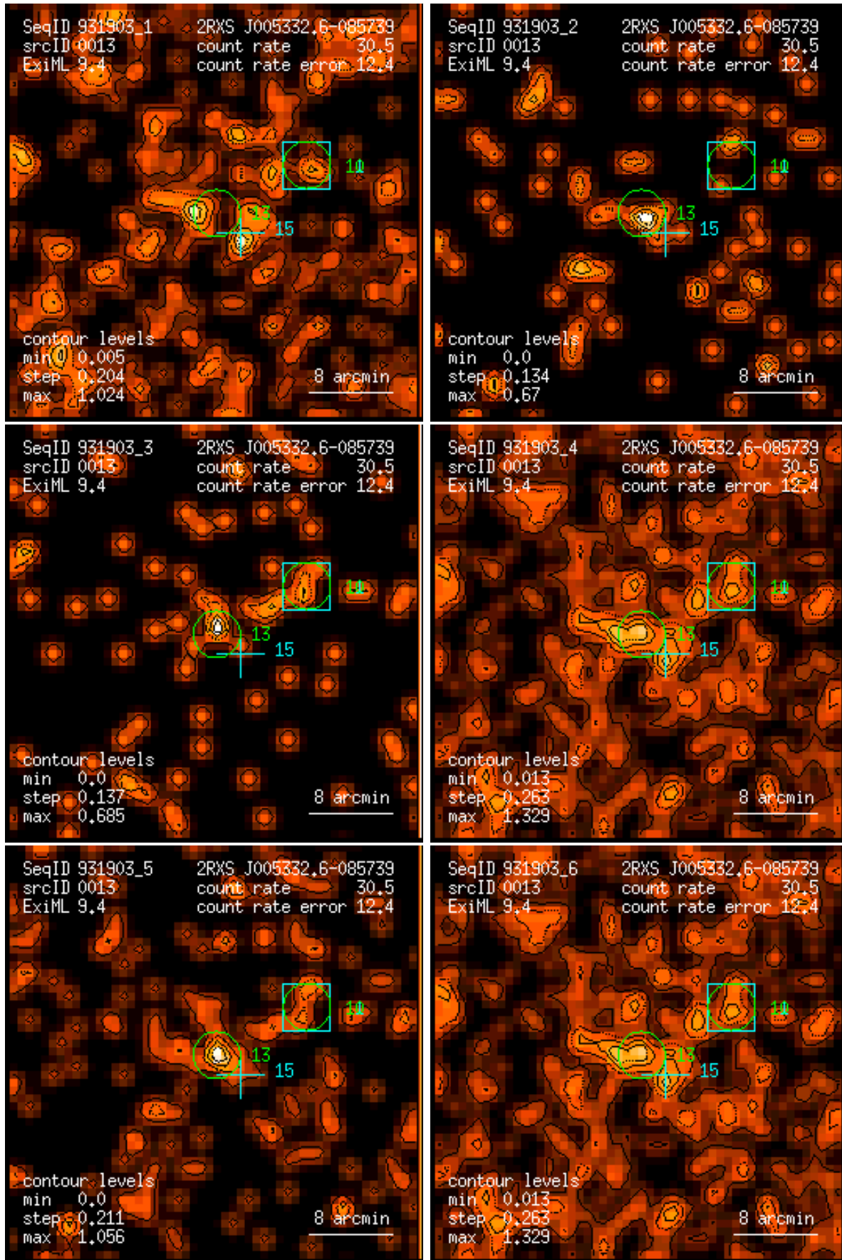
Figure 13: RASS 931903: detection 0013: band rate images, Gaussian filter: (1) PSPC channels 11 – 41, (2) 52 – 90, (3) 91 – 201, (4) 11 – 235, (5) 52 – 201, (6) 11 – 201. Broad band rates in counts/ks. Band rate contour levels in counts/ks/arcmin 2 .
