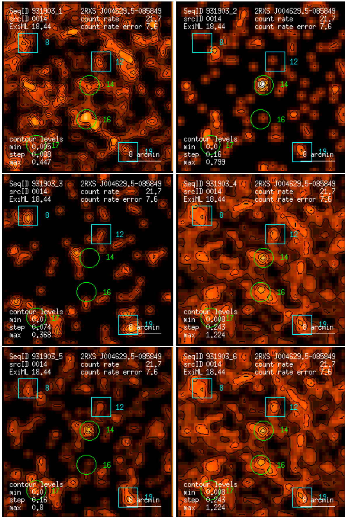
Figure 14: RASS 931903: detection 0014: band rate images, Gaussian filter: (1) PSPC channels 11 – 41, (2) 52 – 90, (3) 91 – 201, (4) 11 – 235, (5) 52 – 201, (6) 11 – 201. Broad band rates in counts/ks. Band rate contour levels in counts/ks/arcmin 2 .
