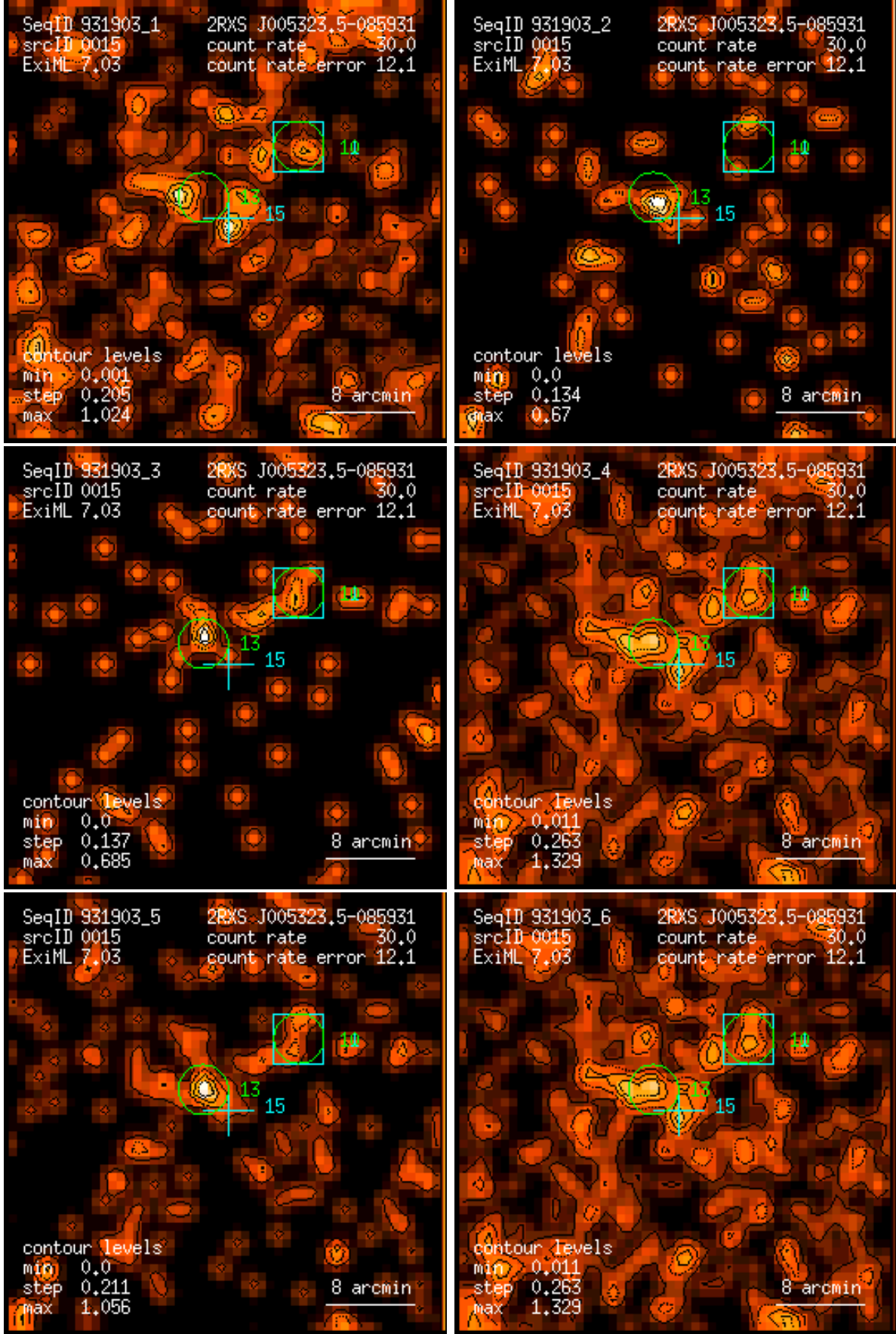
Figure 15: RASS 931903: detection 0015: band rate images, Gaussian filter: (1) PSPC channels 11 – 41, (2) 52 – 90, (3) 91 – 201, (4) 11 – 235, (5) 52 – 201, (6) 11 – 201. Broad band rates in counts/ks. Band rate contour levels in counts/ks/arcmin 2 .
