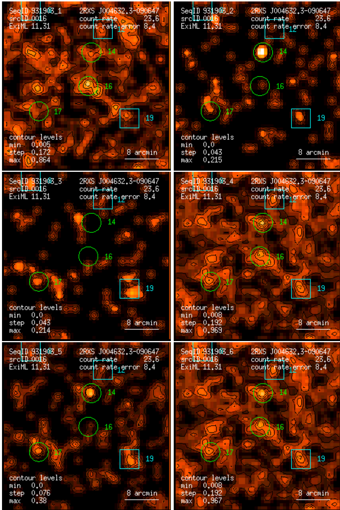
Figure 16: RASS 931903: detection 0016: band rate images, Gaussian filter: (1) PSPC channels 11 – 41, (2) 52 – 90, (3) 91 – 201, (4) 11 – 235, (5) 52 – 201, (6) 11 – 201. Broad band rates in counts/ks. Band rate contour levels in counts/ks/arcmin 2 .
