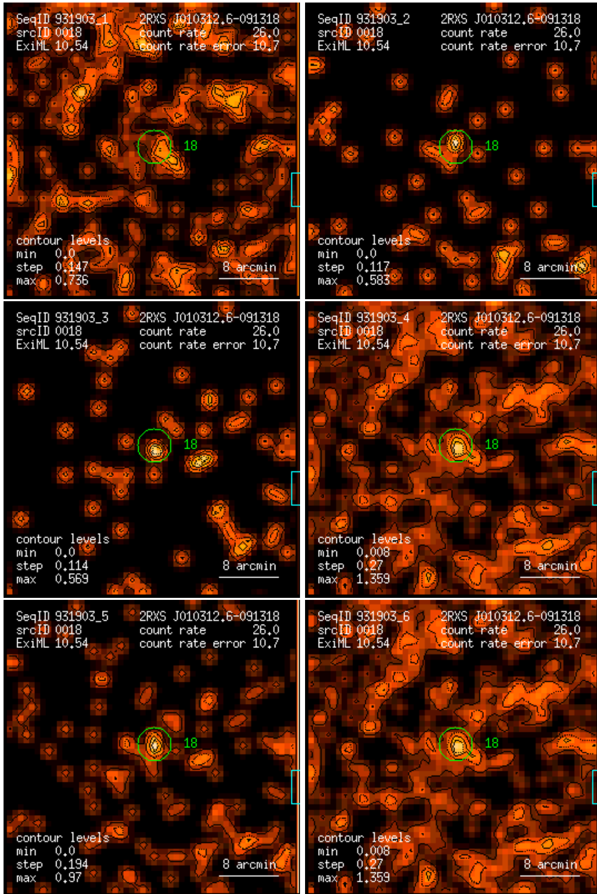
Figure 18: RASS 931903: detection 0018: band rate images, Gaussian filter: (1) PSPC channels 11 – 41, (2) 52 – 90, (3) 91 – 201, (4) 11 – 235, (5) 52 – 201, (6) 11 – 201. Broad band rates in counts/ks. Band rate contour levels in counts/ks/arcmin 2 .
