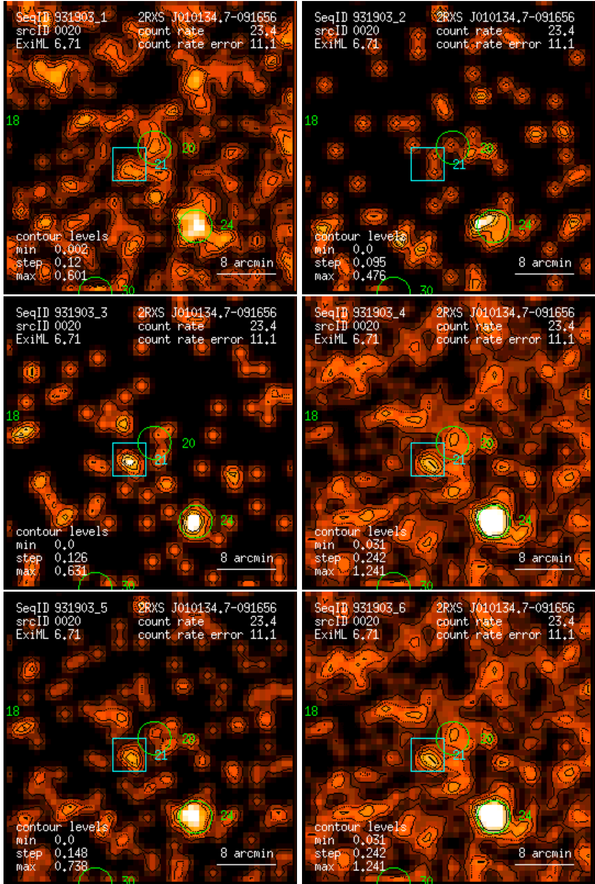
Figure 20: RASS 931903: detection 0020: band rate images, Gaussian filter: (1) PSPC channels 11 – 41, (2) 52 – 90, (3) 91 – 201, (4) 11 – 235, (5) 52 – 201, (6) 11 – 201. Broad band rates in counts/ks. Band rate contour levels in counts/ks/arcmin 2 .
