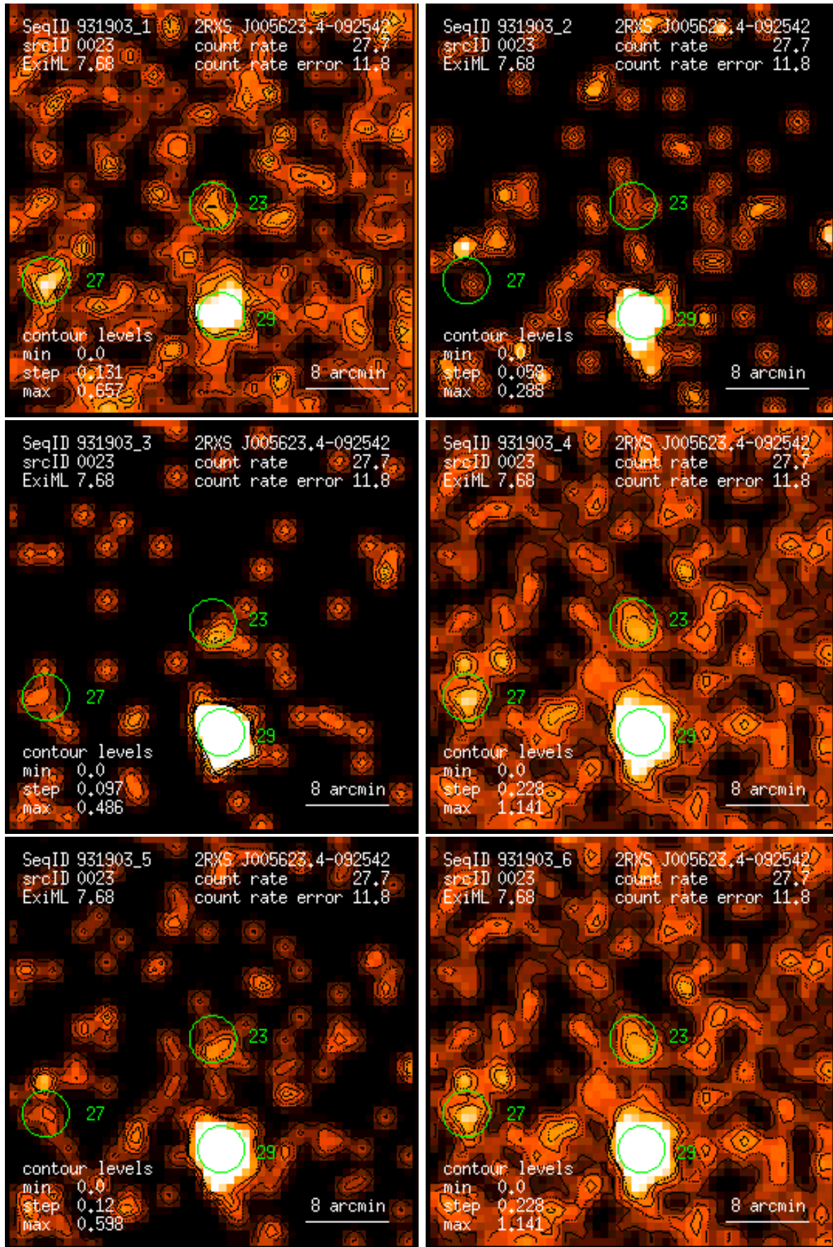
Figure 23: RASS 931903: detection 0023: band rate images, Gaussian filter: (1) PSPC channels 11 – 41, (2) 52 – 90, (3) 91 – 201, (4) 11 – 235, (5) 52 – 201, (6) 11 – 201. Broad band rates in counts/ks. Band rate contour levels in counts/ks/arcmin 2 .
