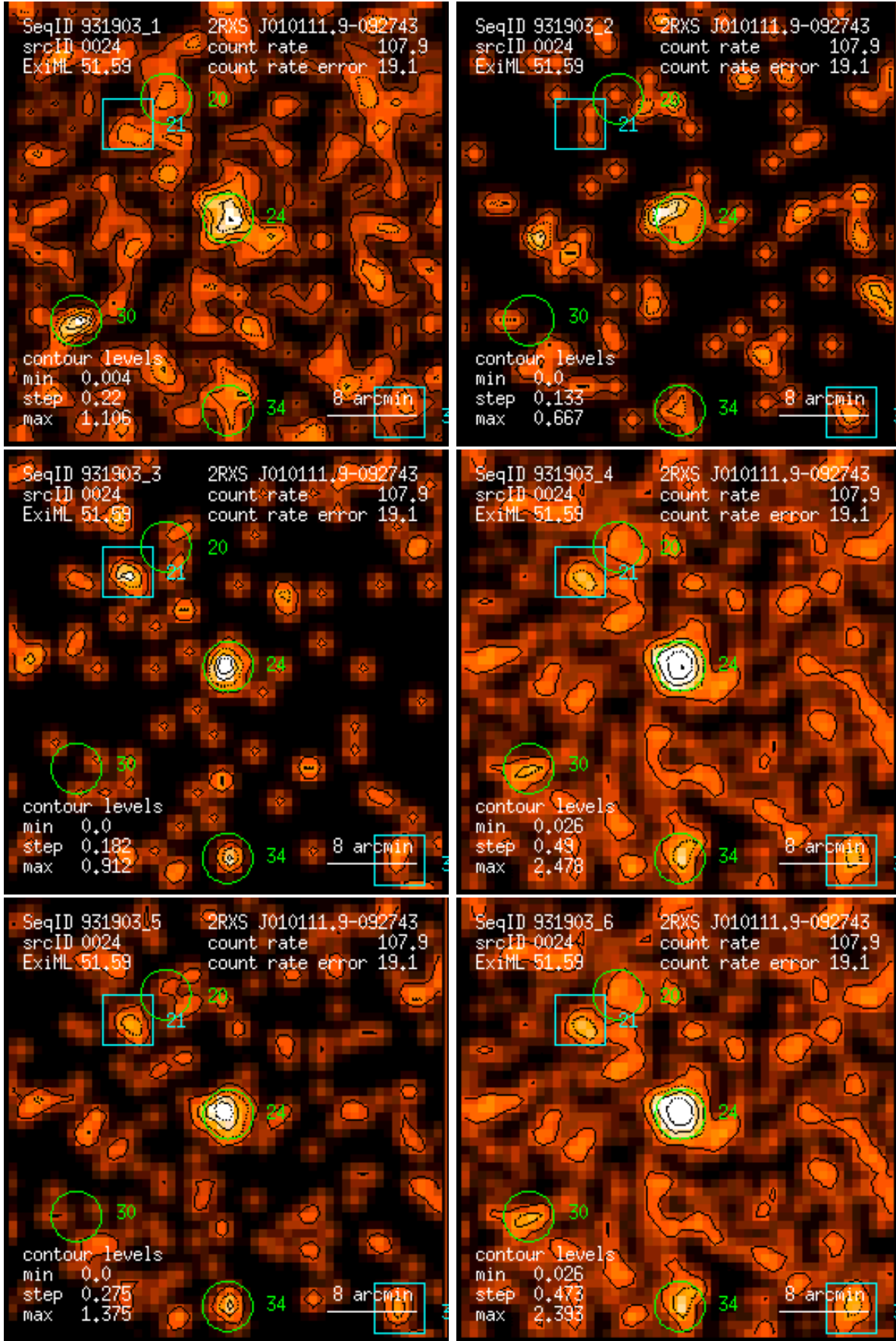
Figure 24: RASS 931903: detection 0024: band rate images, Gaussian filter: (1) PSPC channels 11 – 41, (2) 52 – 90, (3) 91 – 201, (4) 11 – 235, (5) 52 – 201, (6) 11 – 201. Broad band rates in counts/ks. Band rate contour levels in counts/ks/arcmin 2 .
