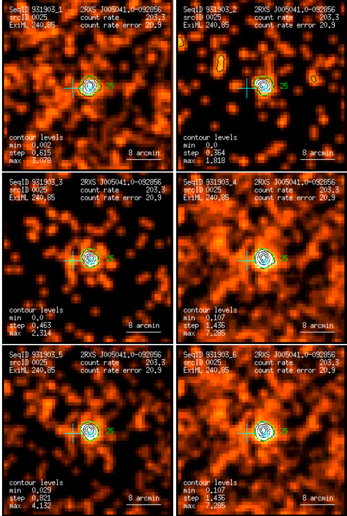
Figure 25: RASS 931903: detection 0025: band rate images, Gaussian filter: (1) PSPC channels 11 – 41, (2) 52 – 90, (3) 91 – 201, (4) 11 – 235, (5) 52 – 201, (6) 11 – 201. Broad band rates in counts/ks. Band rate contour levels in counts/ks/arcmin 2 .
