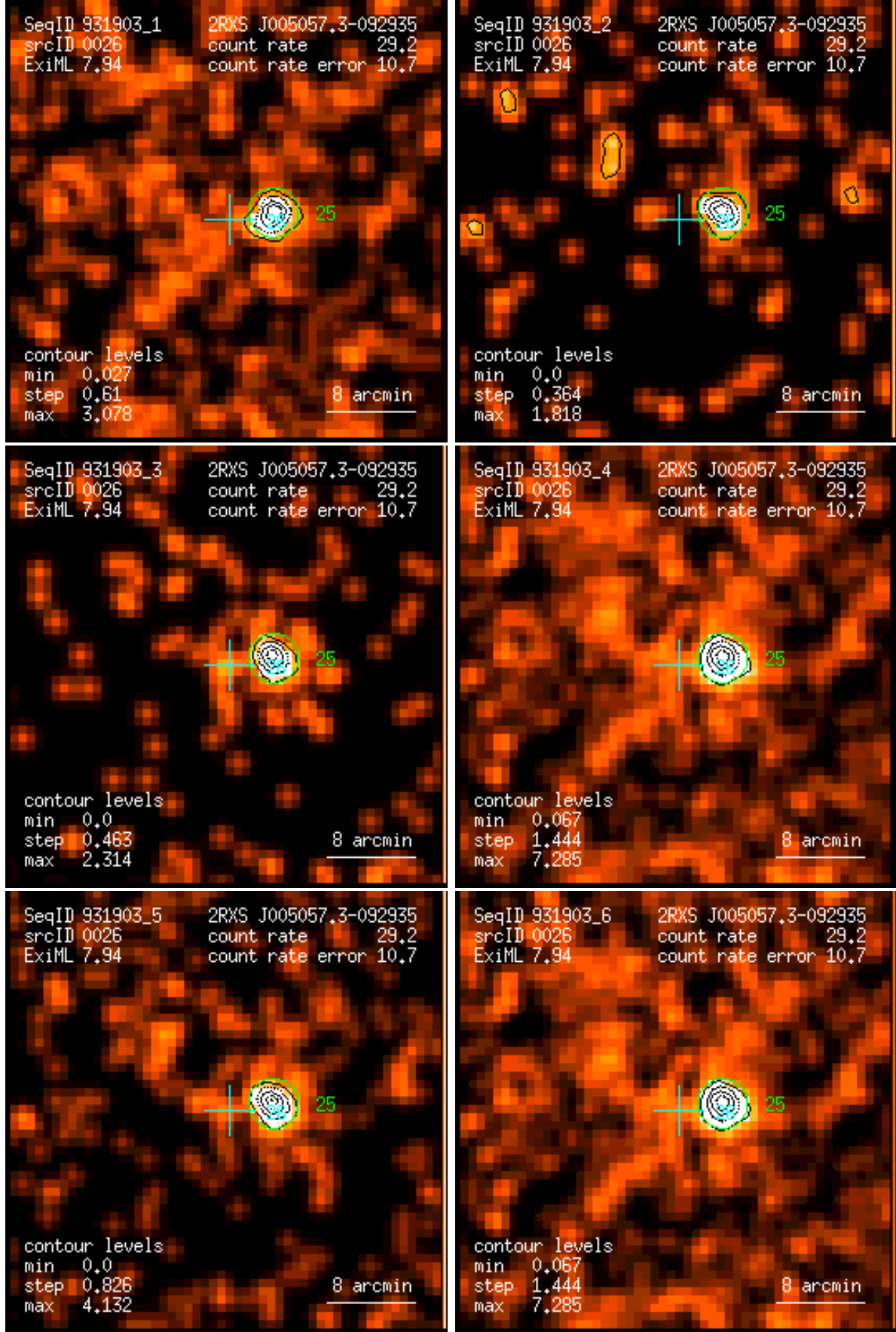
Figure 26: RASS 931903: detection 0026: band rate images, Gaussian filter: (1) PSPC channels 11 – 41, (2) 52 – 90, (3) 91 – 201, (4) 11 – 235, (5) 52 – 201, (6) 11 – 201. Broad band rates in counts/ks. Band rate contour levels in counts/ks/arcmin 2 .
