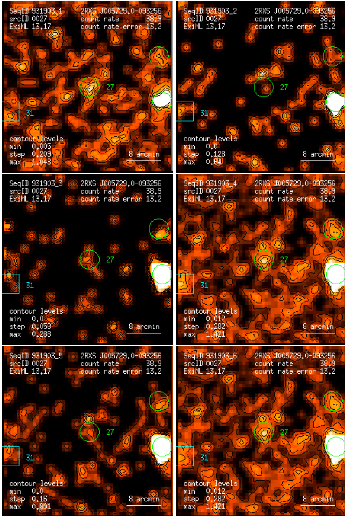
Figure 27: RASS 931903: detection 0027: band rate images, Gaussian filter: (1) PSPC channels 11 – 41, (2) 52 – 90, (3) 91 – 201, (4) 11 – 235, (5) 52 – 201, (6) 11 – 201. Broad band rates in counts/ks. Band rate contour levels in counts/ks/arcmin 2 .
