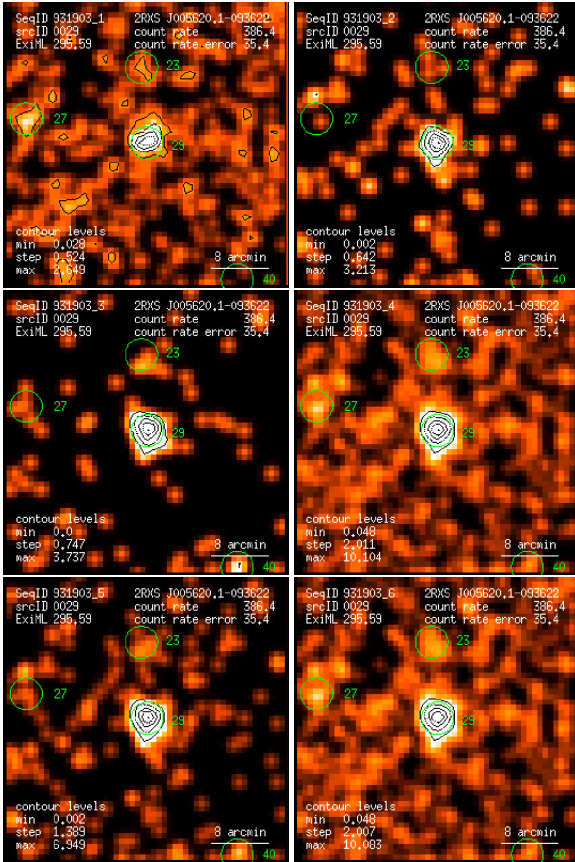
Figure 29: RASS 931903: detection 0029: band rate images, Gaussian filter: (1) PSPC channels 11 – 41, (2) 52 – 90, (3) 91 – 201, (4) 11 – 235, (5) 52 – 201, (6) 11 – 201. Broad band rates in counts/ks. Band rate contour levels in counts/ks/arcmin 2 .
