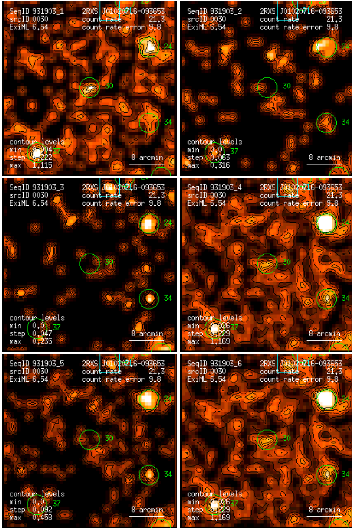
Figure 30: RASS 931903: detection 0030: band rate images, Gaussian filter: (1) PSPC channels 11 – 41, (2) 52 – 90, (3) 91 – 201, (4) 11 – 235, (5) 52 – 201, (6) 11 – 201. Broad band rates in counts/ks. Band rate contour levels in counts/ks/arcmin 2 .
