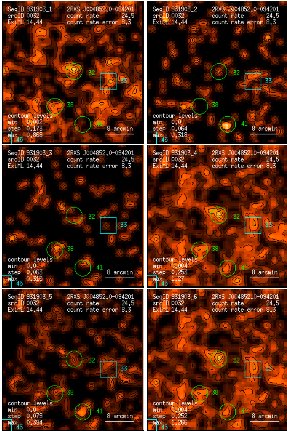
Figure 32: RASS 931903: detection 0032: band rate images, Gaussian filter: (1) PSPC channels 11 – 41, (2) 52 – 90, (3) 91 – 201, (4) 11 – 235, (5) 52 – 201, (6) 11 – 201. Broad band rates in counts/ks. Band rate contour levels in counts/ks/arcmin 2 .
