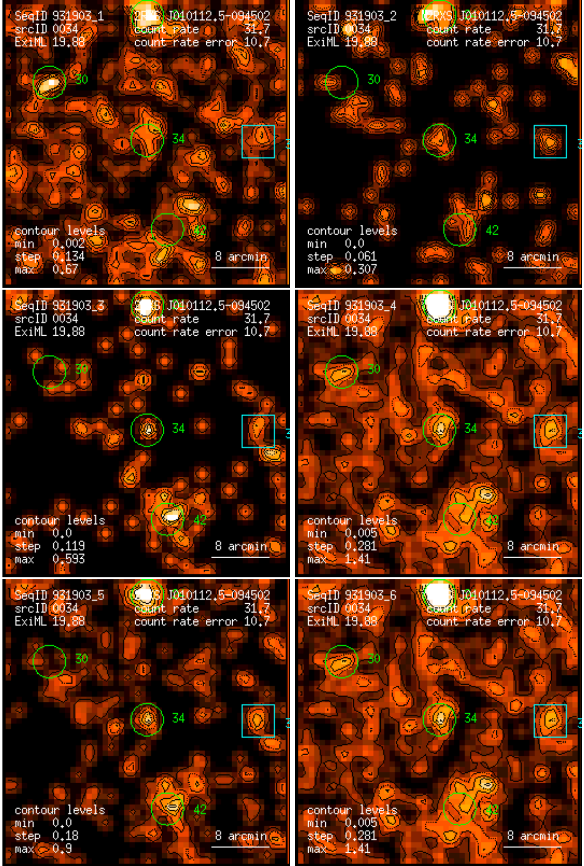
Figure 34: RASS 931903: detection 0034: band rate images, Gaussian filter: (1) PSPC channels 11 – 41, (2) 52 – 90, (3) 91 – 201, (4) 11 – 235, (5) 52 – 201, (6) 11 – 201. Broad band rates in counts/ks. Band rate contour levels in counts/ks/arcmin 2 .
