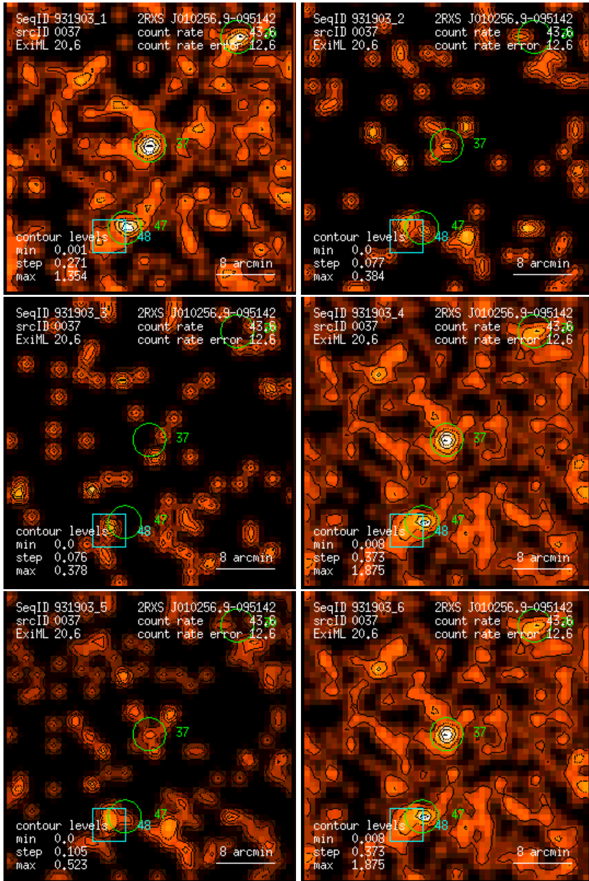
Figure 37: RASS 931903: detection 0037: band rate images, Gaussian filter: (1) PSPC channels 11 – 41, (2) 52 – 90, (3) 91 – 201, (4) 11 – 235, (5) 52 – 201, (6) 11 – 201. Broad band rates in counts/ks. Band rate contour levels in counts/ks/arcmin 2 .
